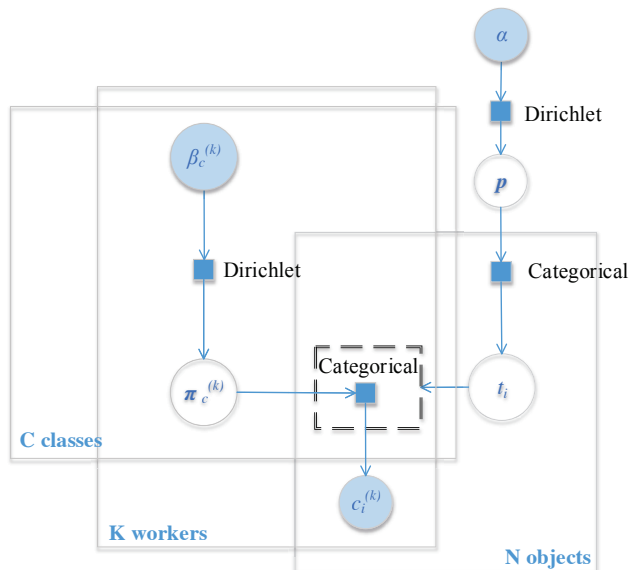
Figure 1: The factor graph of BCC. The users plate includes the user's confusion matrix \pi^{(k)} while the objects plate includes the true object class variable t_i . The observed (shaded) user's vote c_i^{(k)} lies at their intersection
