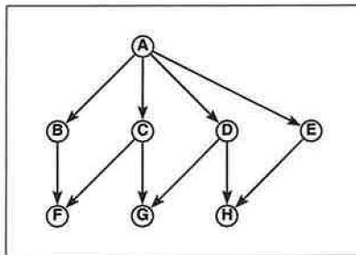
Figure 11 Type hierarchy.
