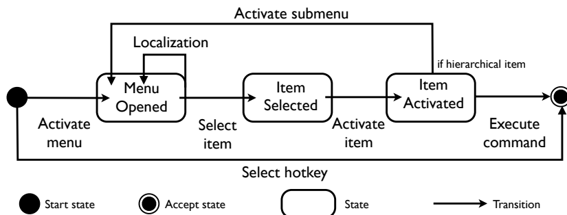
Figure 1: Command execution process in a menu system.
