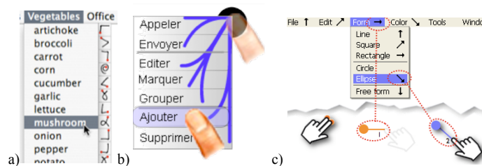
Figure 21: Command-gesture mapping displayed a) [Appert et al. 2009], b) Leaf menus [Roudaut et al. 2009], c) Radial-Stroke shortcuts [Bailly et al 2010], @ACM.
