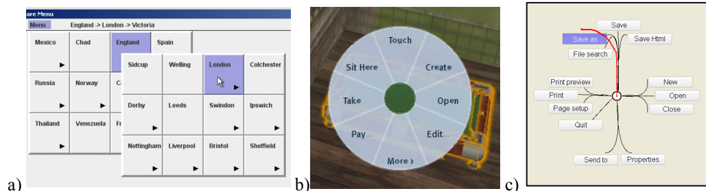
Figure 13: a) Square menus [Ahlstrom et al. 2010], © ACM, organize items in a matrix. b) Pie menus [Callahan et al. 1988], © ACM, place items in a circular design at an equal radial distance from the center (radial layout) .c) Flower menus [Bailly et al. 2008] are a variant of Marking menus which rely on curved gestures to increase the number of commands.
