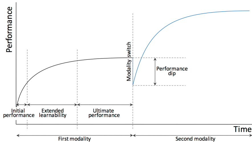
Figure 9. Framework of interface expertise [Scarr et al. 2012], © ACM, showing the transition from the menu (first modality) to the second modality (expert mode).
