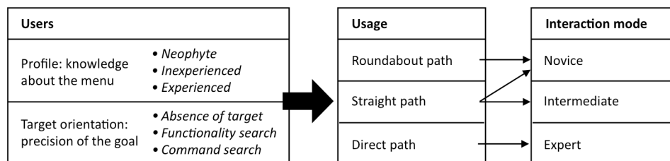
Figure 4: Modes of a menu according to users’ profile and their goals.
