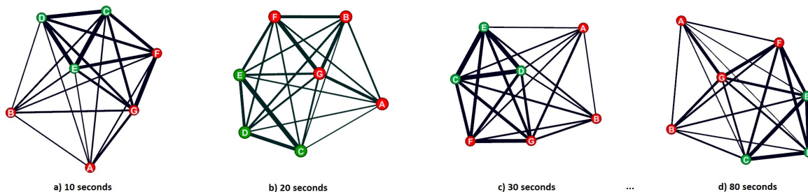
Figure 9: Community network graph rendered with ForceAtlas 2, with data over time from 10, 20, 30, and 80 seconds. Taken from the interaction "Experiment 2" from the conference scenario in Table 1, nodes coloured by a modularity of 0.8.
