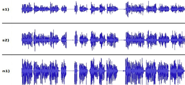
Figure 5: Sound waveforms captured by two Samsung S5 devices "s1", "s2" and a Nexus 5 "n1" recording the same speech segments at the same distance from the source. The devices have different gains.
