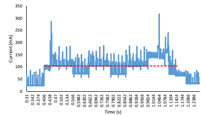
Figure 15: Current over time for one Wi-Fi scan
