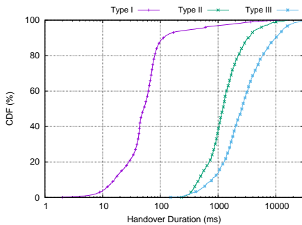
Figure 12: Handover Duration.
