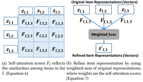
Figure 3: Refining item representations ( z_{l1} ) by considering the consistency with neighboring items (i.e., z_{l2} and z_{l3} ).
