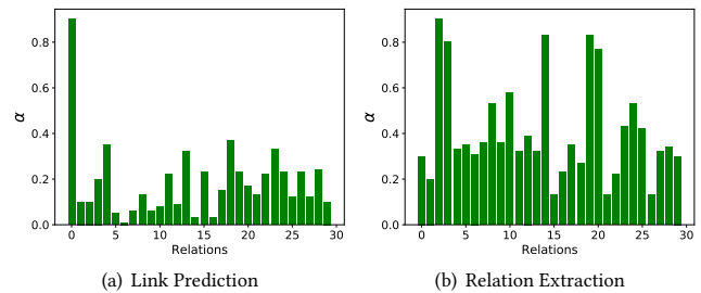
Figure 7: \alpha w.r.t #Relations.
