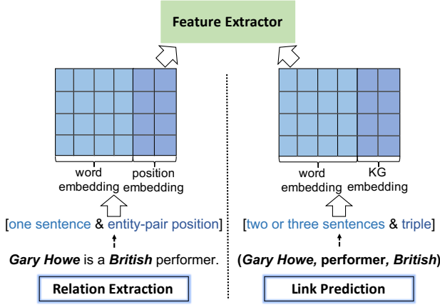
Figure 4: Instance Encoder.
