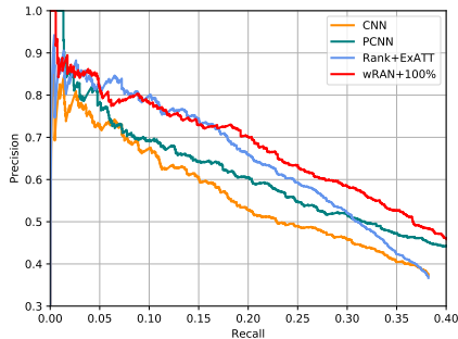
Figure 6: Supervised adaptation results.
