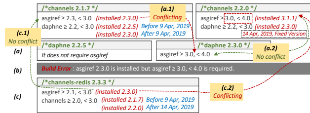
Figure 1: Illustrative examples of dependency conflict issues
