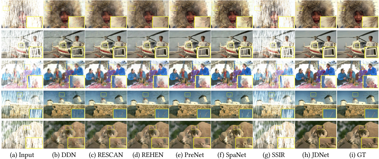
Figure 6: Examples about the comparison of our method with other methods on Rain100H dataset.
