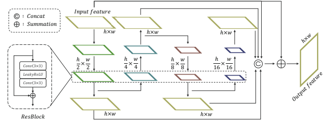
Figure 4: Scale-Aggregation Module.
