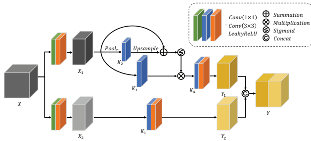
Figure 5: Self-Calibrated Convolution.
