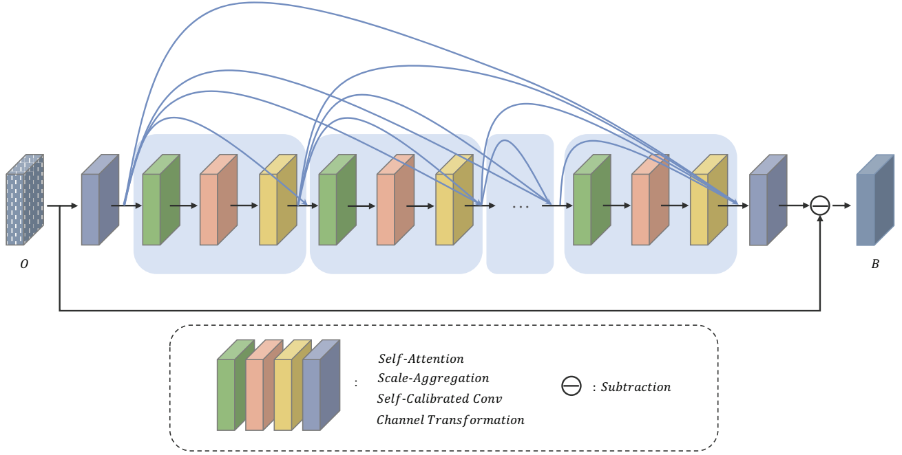
Figure 2: The architecture of Joint Network for deraining (JDNet). Each joint unit is composed of a Self-Attention module, Scale-Aggregation layer and Self-Calibrated convolution. We use dense connections to inner-connect several joint units. And at the first layer and last layer, we use 3 \times 3 convolution following a LeakyReLU to change the channel dimensions.
