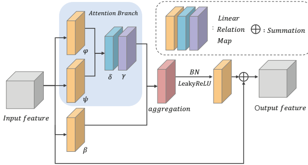
Figure 3: The architecture of Pairwise Self-Attention Module.
