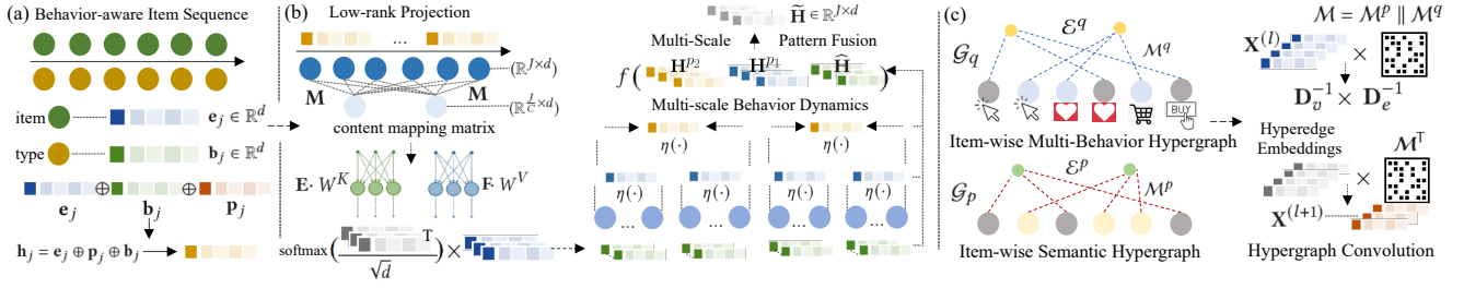
Figure 2: MBHT’s model flow. (a) We inject the behavior-aware interaction context into item embeddings \mathbf{h}_j = \mathbf{e}_j \oplus \mathbf{p}_j \oplus \mathbf{b}_j . (b) Multi-scale transformer architecture to capture behavior-aware transitional patterns via low-rank self-attention and multi-scale sequence aggregation. Scale-specific behavior patterns are fused through the fusion function \tilde{\mathbf{H}} = f(\hat{\mathbf{H}} \parallel \mathbf{H}^{p_1} \parallel \mathbf{H}^{p_2}) . (c) We capture the global and personalized multi-behavior dependency learning with our hypergraph neural architecture over \mathcal{G} .
