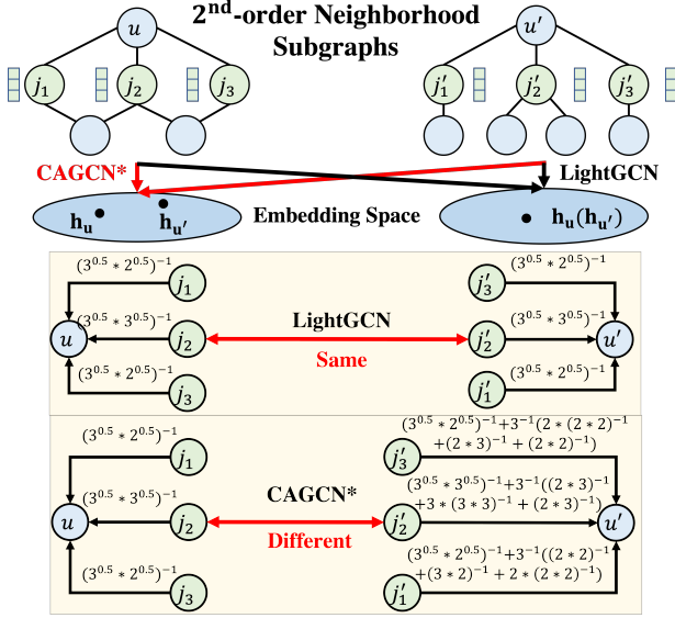
Figure 11: An example showing two neighborhood subgraph S_u, S_{u'} that are subgraph-isomorphic but not bipartite-subgraph-isomorphic.
