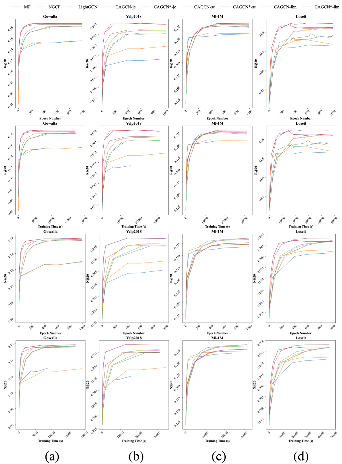
Figure 12: Comparing the training efficiency of each model under R@20 and N@20.
