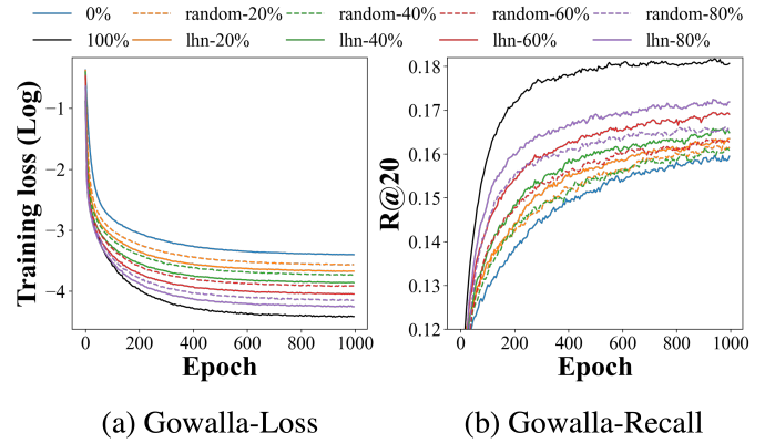
Figure 2: The training loss (left) is lower and the performance (right) is higher when adding edges according to the variant CIR-lhn (Leicht Holme Nerman) than adding randomly under the same addition budget. Detailed experimental settings and more results are provided in Appendix A.5.1.
