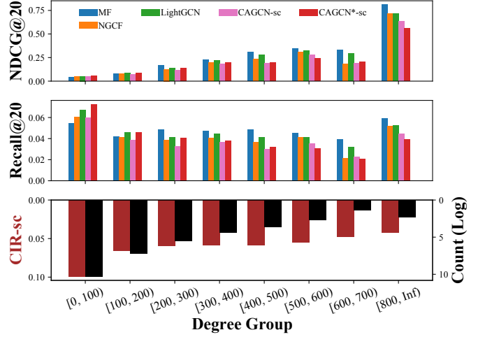
Figure 10: Performance of model w.r.t. node degree on Yelp.
