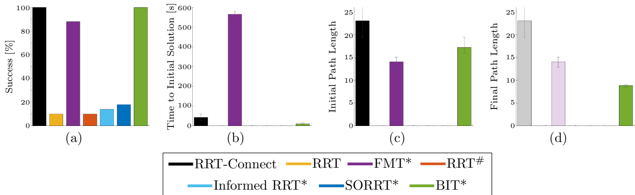
Figure 14. Results from 50, 600 second trials on the two-armed HERB planning problem shown in Fig. 13. The percent of solutions solved, (a), the median time to an initial solution, (b), the median initial path length, (c), and the median final path length, (d), are presented with 99% confidence intervals for each planner. Unsuccessful trials were assigned infinite time and cost. The inability of nonanytime planners (e.g., RRT, RRT-Connect, and FMT*) to use the remaining available time to improve their initial solution is denoted with diminished colour in (d), when present. BIT* is the only anytime planner to solve all 50 trials and does so in a time comparable to RRT-Connect. It focuses the search to the informed set once a solution is found and the resulting increasingly dense RGG allows it to find lower cost paths than all the other planners.
