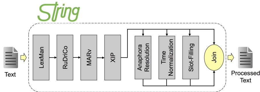
Fig. 1. STRING Architecture (from [34]).
