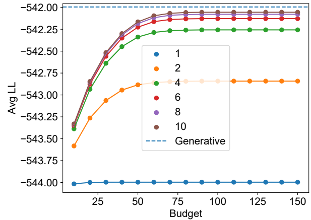
Figure 2: Budget versus Log Likelihood, Generative Classifier
