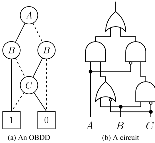
Figure 1: An OBDD and circuit representation of a linear classifier A + B - C \geq \frac{1}{2} .
