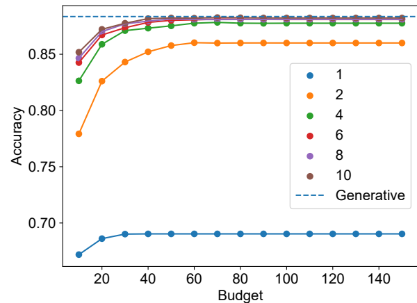
Figure 3: Budget versus Accuracy, Generative Classifier
