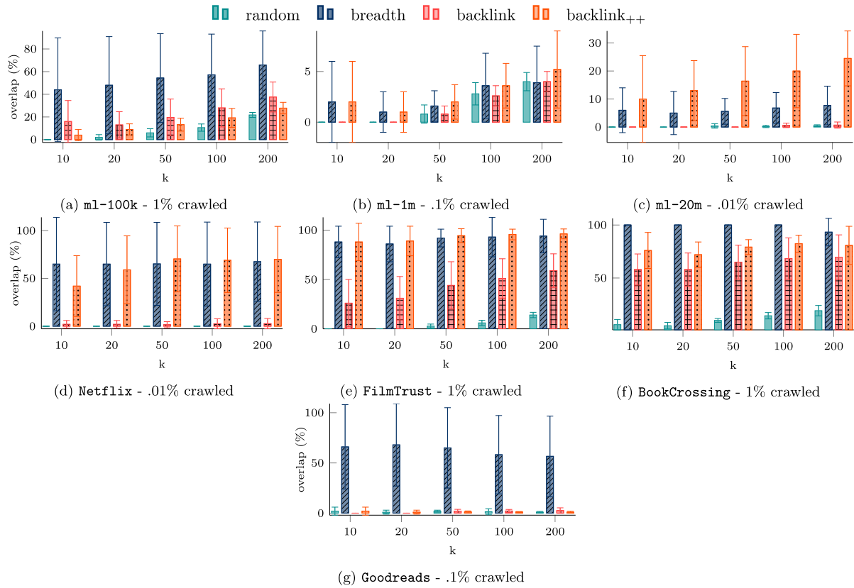
Fig. 7. Neighborhood reconstruction using user-based cosine similarity. The results are the average ( \pm standard deviation) over five randomly selected users. k on the x -axis is the dimension of the considered neighborhood.
