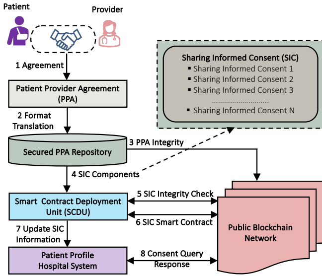
Fig. 3. SIC Smart Contract Deployment Process.
