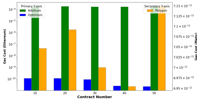
Fig. 13. Contract Deployment Gas Cost.
