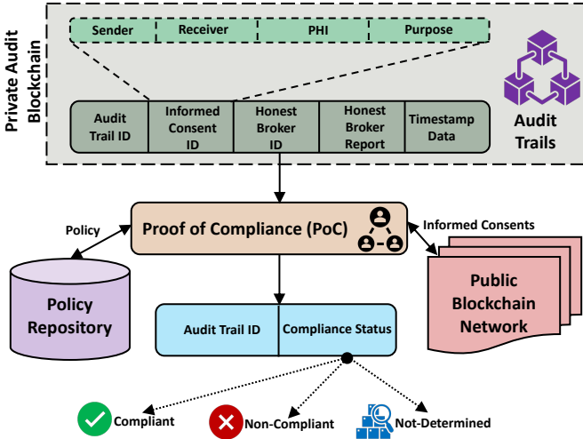
Fig. 7. Proof of Compliance (PoC) Transaction Structure.
