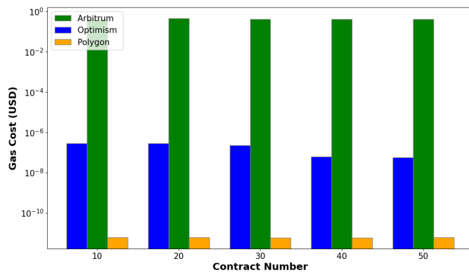
Fig. 14. Contract Deployment USD Cost.
