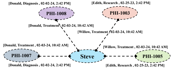
Fig. 10. Receiver-Oriented Executed Consents.
