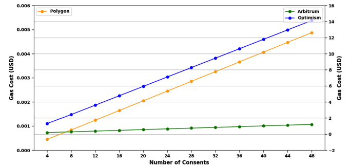
Fig. 16. Consent Storage USD Cost.
