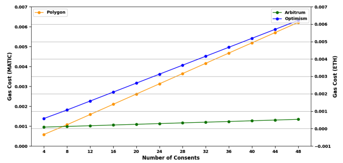
Fig. 15. Consent Storage Gas Cost.
