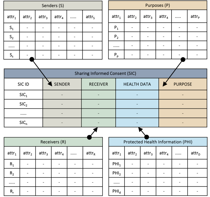
Fig. 2. Sharing Informed Consent (SIC) Structure.
