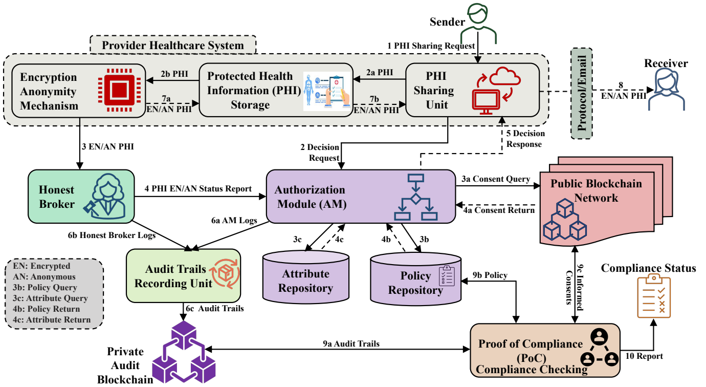
Fig. 4. Compliance-Based PHI Sharing Authorization Process.
