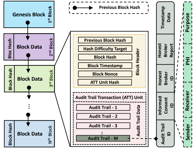
Fig. 5. Audit Blockchain Block Structure.
