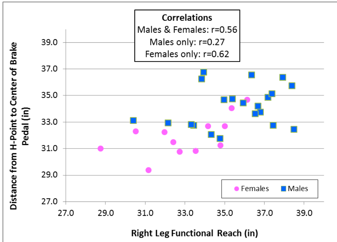
Figure 18. Scatter plot and correlations for right leg functional reach vs. H-point to brake distance, by sex, and for all participants (n=33).
