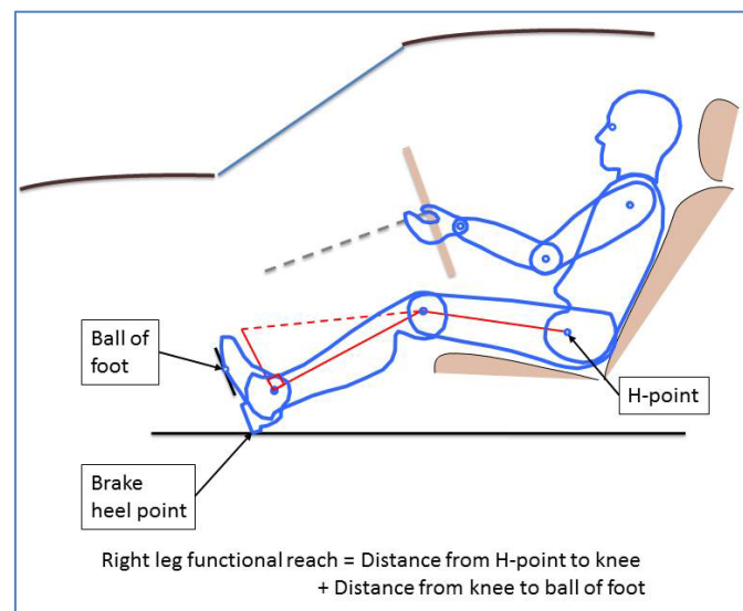
Figure 15. Dimensions used to calculate right leg functional reach length.
