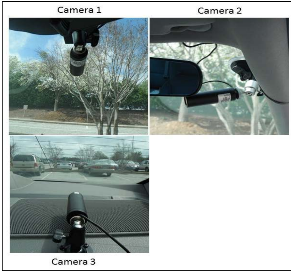
Figure 7. Driver environment cameras.
