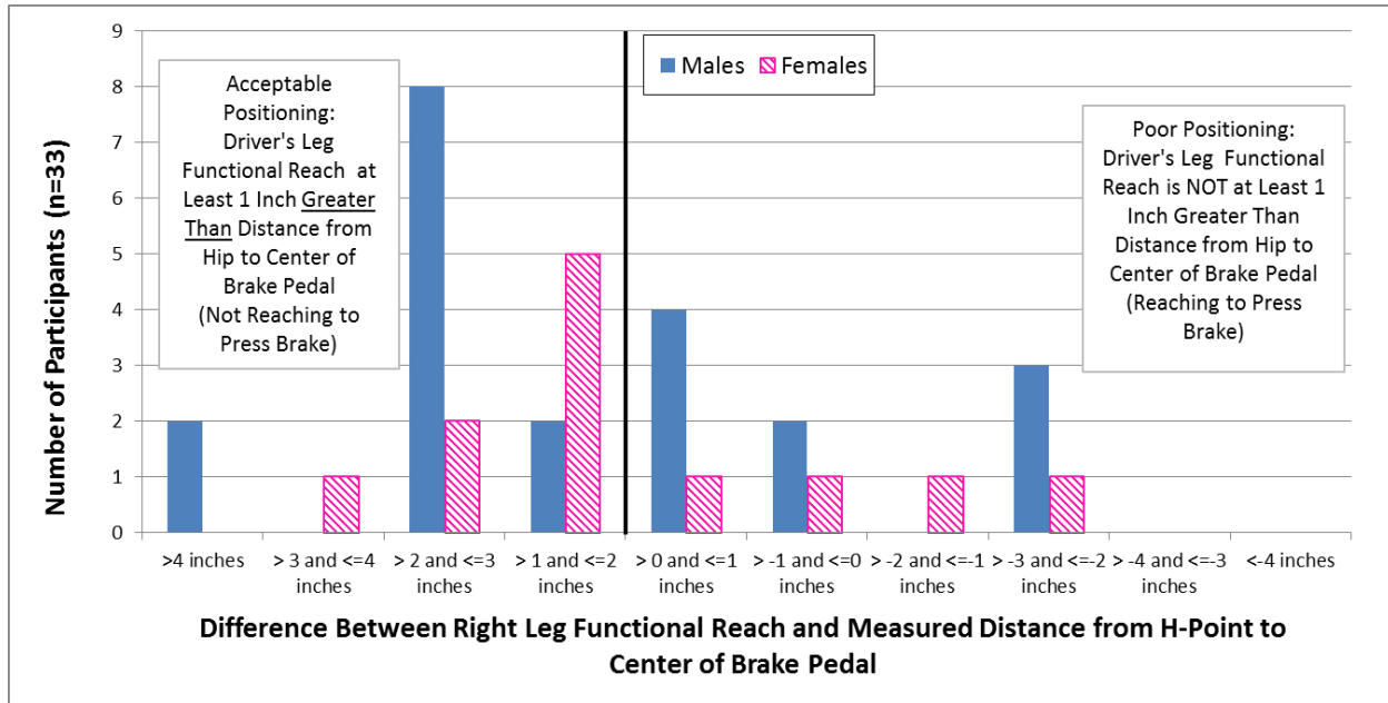
Figure 17. Distribution of the differences between right leg functional reach and distance from H-point to brake, by sex, describing acceptable and poor fit.
