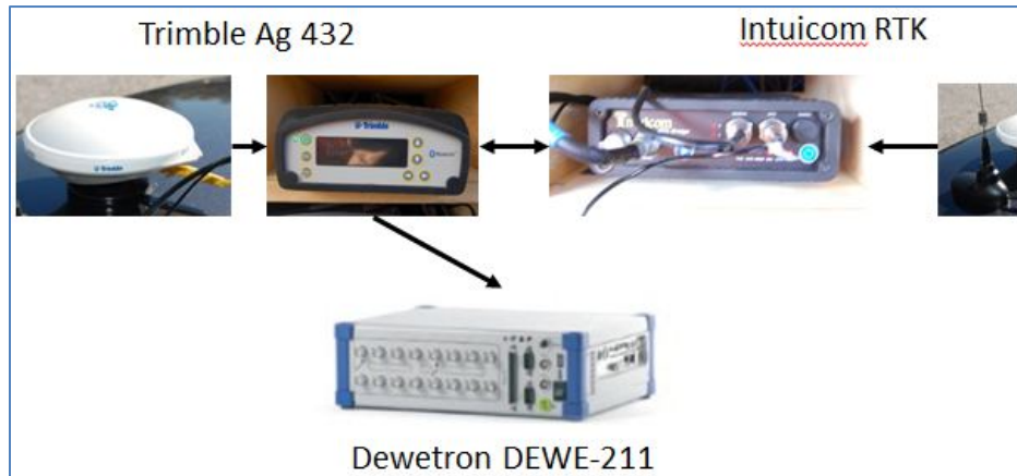
Figure 9. GPS and Dewetron data acquisition components.
