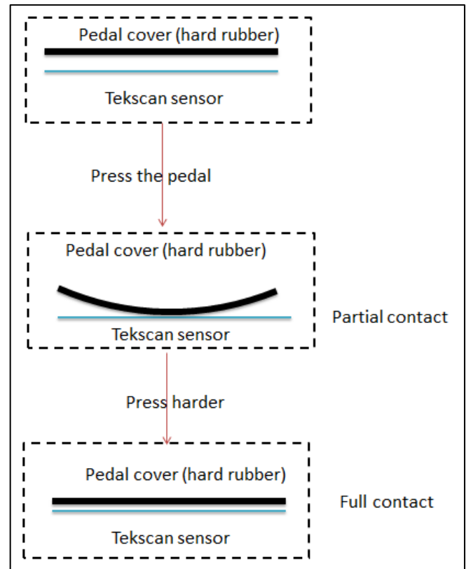
Figure 14. Potential reduction of foot contact area on brake and brake force measures.
