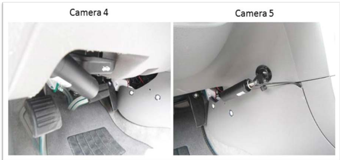
Figure 3. Driver foot well camera location.
