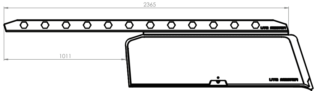
SIDE VIEW CANTILEVER ROOF RACK
