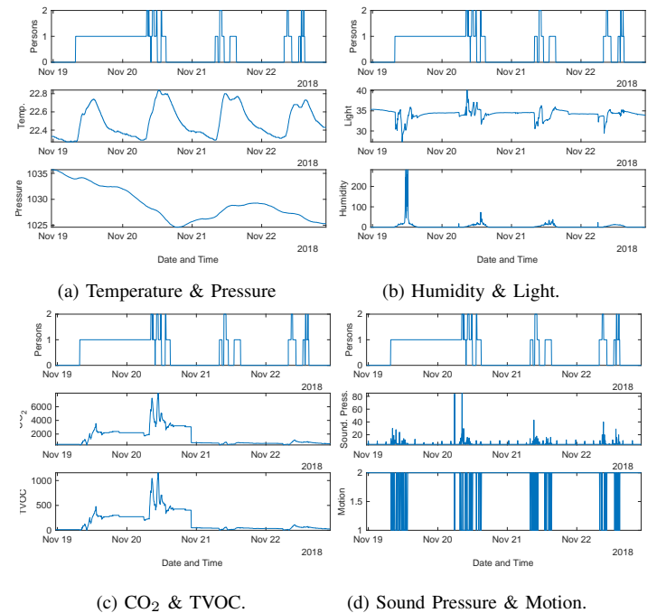
Fig. 3: Variation of environmental parameters from sensor node E2 over a period of about four days.
