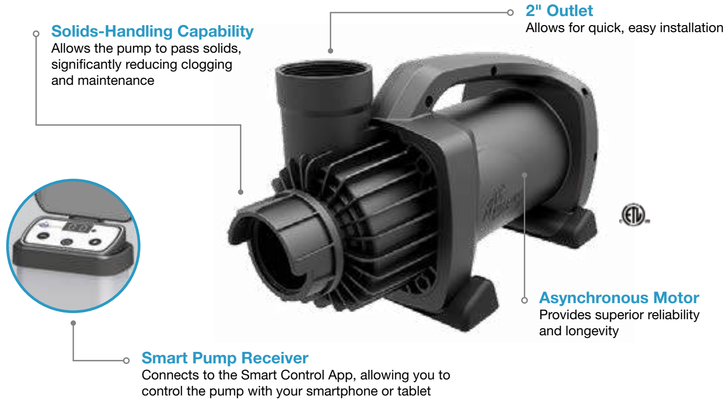
SLD 4000-7000 Adjustable Flow Pond Pump Shown
