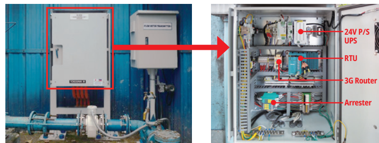
Monitoring box at pumping station
