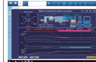
Operator Training Simulator (OTS)
