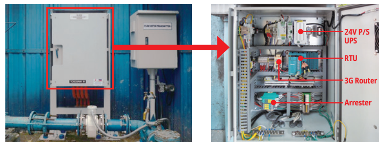
Monitoring box at pumping station
