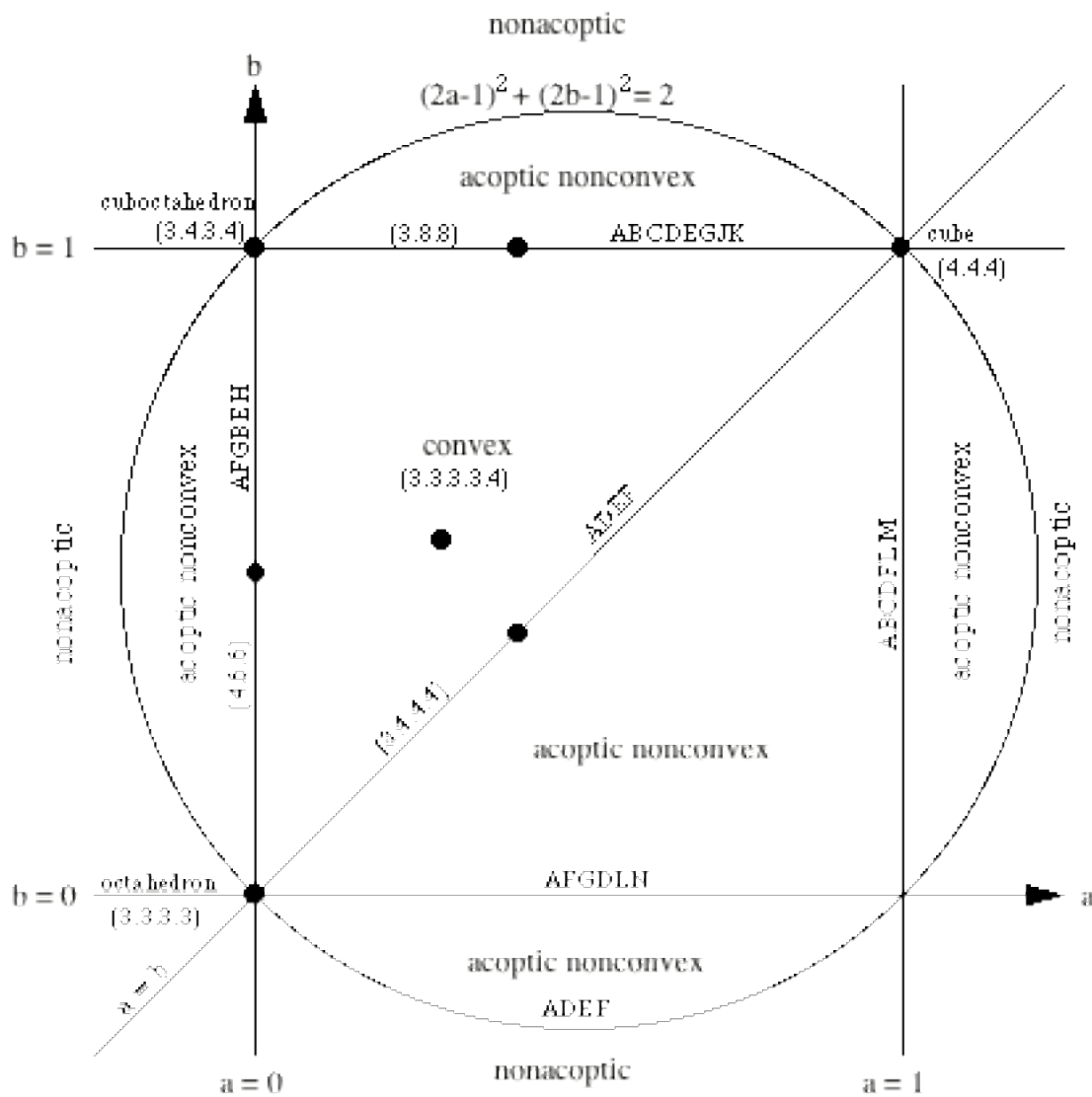
Figure 17. Dynatogram for acoptic isogonal polyhedra of combinatorial type of the snub cube, (3.3.3.3.4) . The parameters a and b determine the coordinates of the vertices, as shown in Figure 16. All regions outside of the large circle correspond to nonacoptic polyhedra, while the polyhedra with parameter values on the circle are weakly acoptic. The strings of capital letters near the lines and the circle indicate (in the notation of Figure 16) examples of sets of coplanar vertices. The symbols for isogonal polyhedra near the lines and near three of the vertices of the square indicate to which isogonal polyhedra the polyhedra of type (3.3.3.3.4) are isomegetic (that is, consist of the same set of points). The solid dots indicate the parameter values for which the polyhedra of type (3.3.3.3.4) are isomegetic to a uniform (Archimedean) polyhedra. The uniform (Archimedean) snub cube (3.3.3.3.4) corresponds to the parameter values a = 0.29955977 , b = 0.5436890 .
