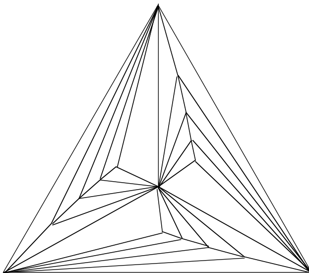
Figure 30. A Schlegel diagram of a convex polyhedron for which no combinatorially equivalent acoptic polyhedron is monohedral.
