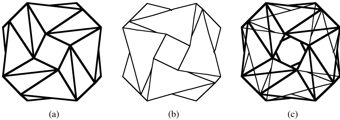
Figure 19. The Boolean sum of the polyhedron in (a) which corresponds to (a,b) = (1/3, 1/6) , with the polyhedron in (b) for which (a,b) = (1/3, -1/6) , yields the isogonal acoptic polyhedron in (c); the elimination of the square faces makes the bottom part of the polyhedron visible in (c). The polyhedron in (c) is a realization of the regular map (3,8)_{12} (which is map #96.162 in Wilson's catalog [W5] of regular maps).
