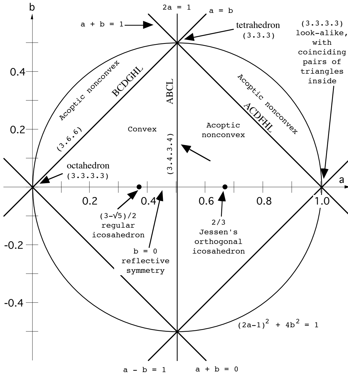
Figure 21. Dynatogram for acoptic isogonal polyhedra of combinatorial type of the icosahedron, (3.3.3.3.3). As shown in Figure 20, the parameters a and b determine the coordinates of the vertices; they are given (in Cartesian coordinates) by all cyclic permutations of (\pm a, \pm(1-a), \pm b) with an even number of minus signs. The similarity of many features of this dynatogram with the dynatogram of snub cubes in Figure 17 is not surprising since icosahedra can be interpreted as "snub tetrahedra". However, since triangles here play the roles played by both triangles and squares in the case of snub cubes, polyhedra corresponding to the bottom part of the dynatogram are congruent mirror images of the polyhedra corresponding to the upper part; polyhedra with b = 0 have mirror-symmetry.
