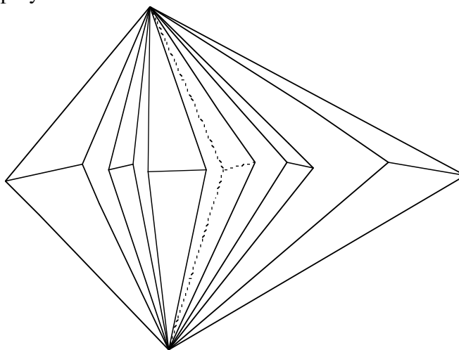
Figure 31. An acoptic polyhedron of genus 0 with no spanning tree of valence \leq 3 .
