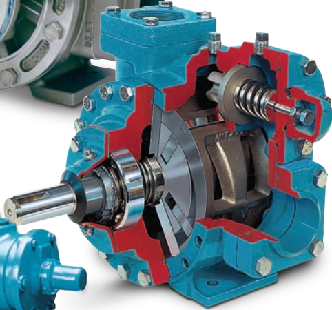
XL Sliding Vane Pump
