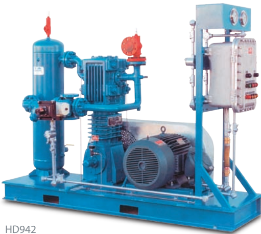
HD942 Liquefied Gas Transfer Compressor Package
