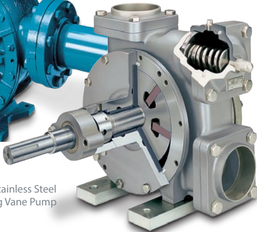
ML Sliding Vane Pump
