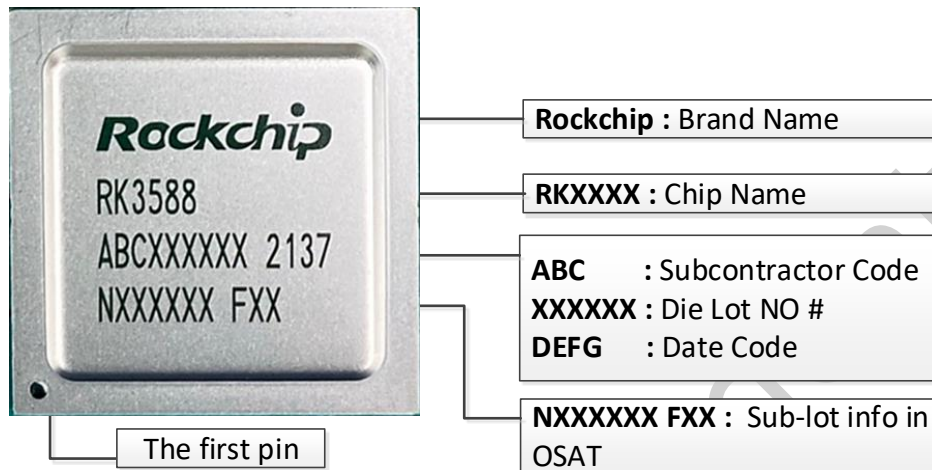
Fig. 2-1 Package definition
