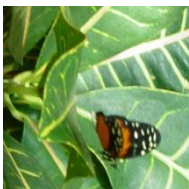
Butterfly – 5 pts
