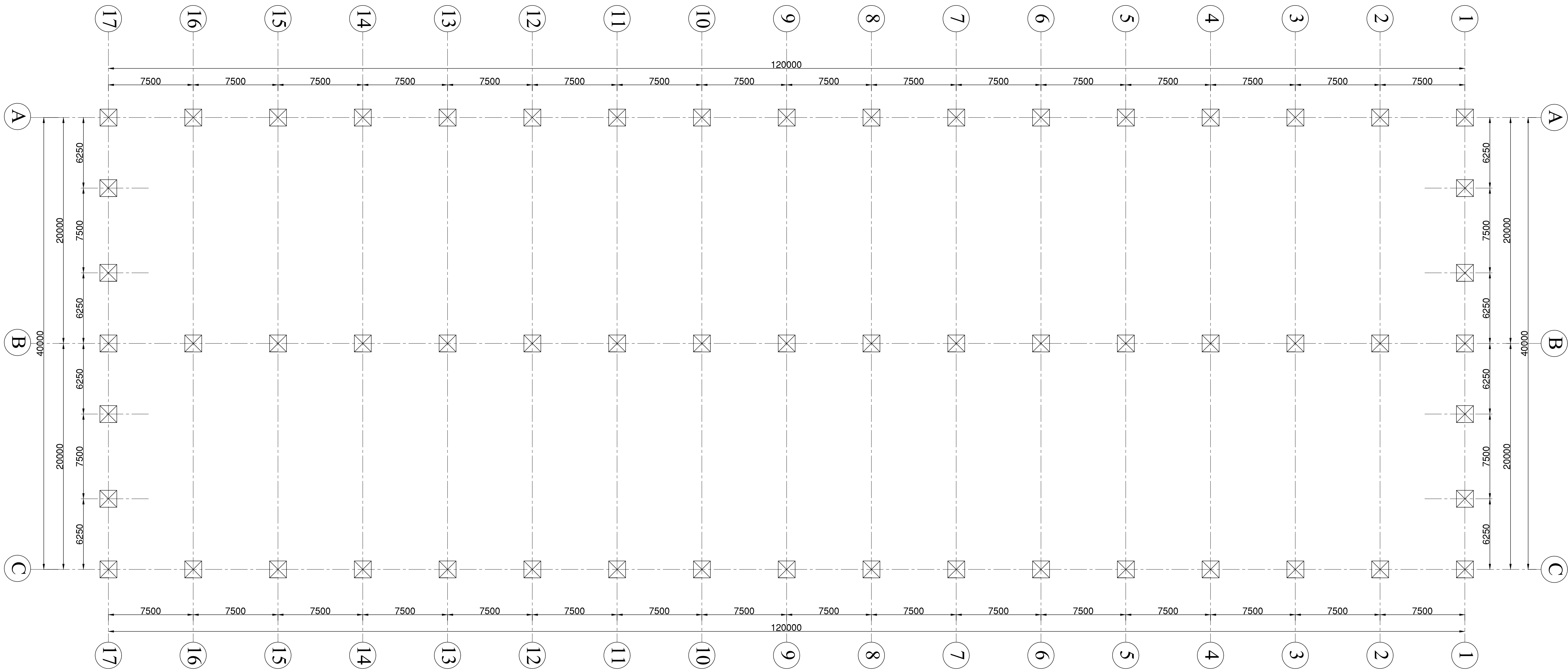
REINFORCED CONCRETE FOUNDATION LAYOUT PLANS SCALE : 1/100
