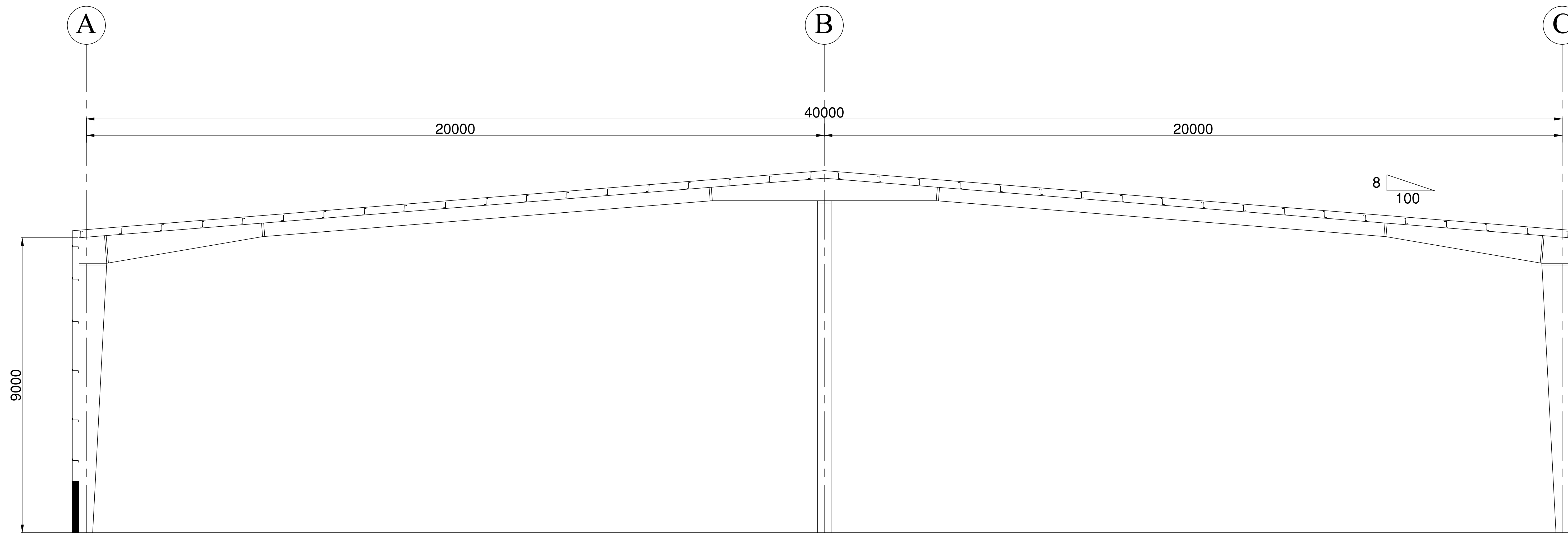
MAIN FRAME SECTION (2-16 AXES)
