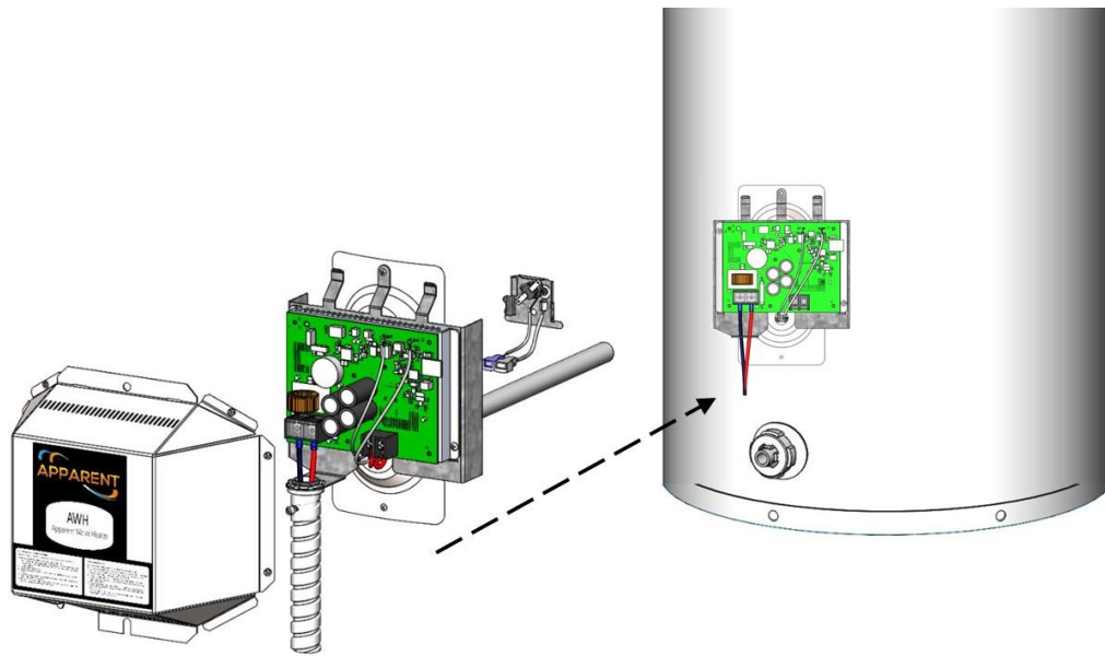
Figure 6. Attached control device using mounting bracket to tank.
