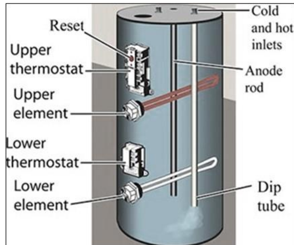
Figure 4. Typical water tank upper and lower thermostats and elements configuration.
