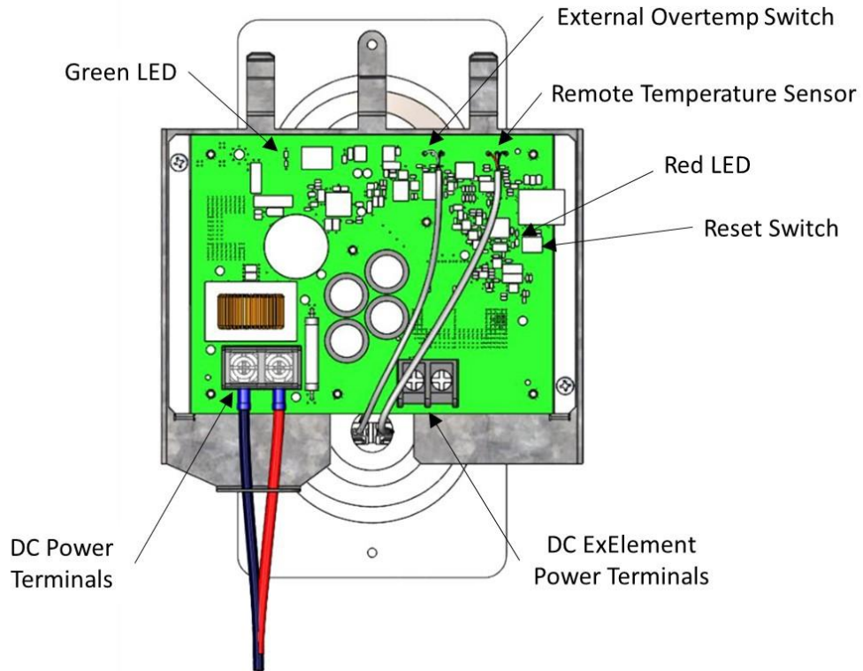
Figure 7. Control device layout (Version 1.x).
