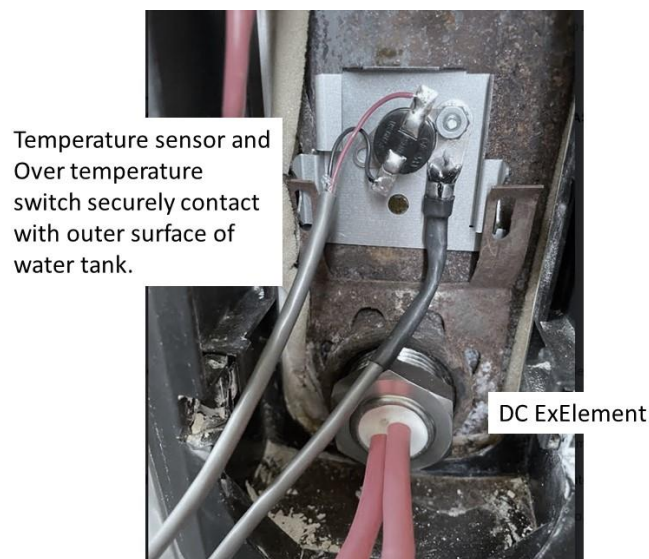
Figure 5. Positioning of ExElement and temperature sensors.
