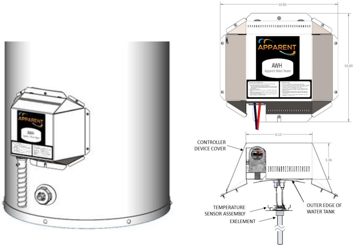
Figure 8. Installed EXEL element and control device with external cover.
