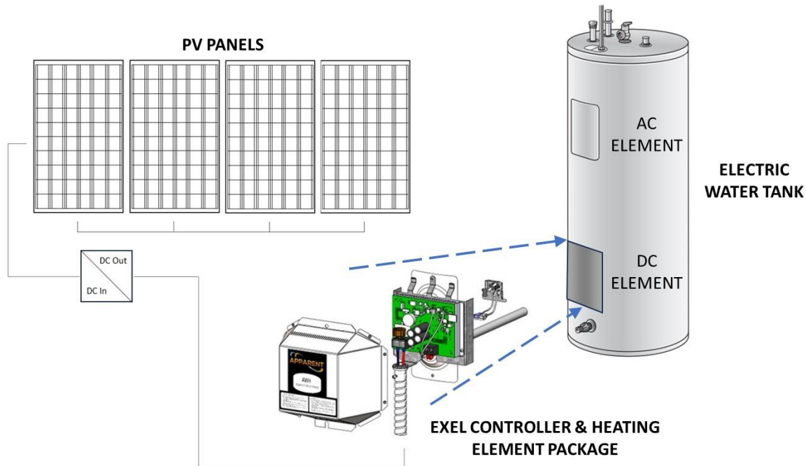
Figure 2. Apparent's EXEL Water Heating System Components in Single DC ExElement configuration.
