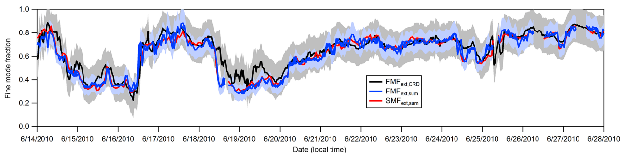
Figure 3. The fine-mode fraction of extinction (SMF and FMF_{ext} ) for the latter half of the campaign at T1. Here, the FMF_{ext,CRD} is determined for particles sampled without a size cut applied. Uncertainty ranges are shown as light colored bands.
