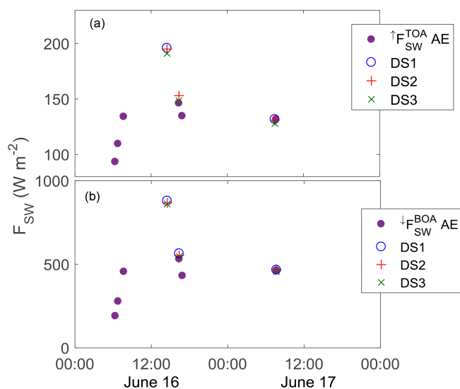
Figure 7. Time series of the \uparrow F_{\text{SW}} at the TOA (a) and \downarrow F_{\text{SW}} at the BOA (b) for the period 16–17 June. The purple dots are AERONET fluxes, and GAME output data for different inputs are represented by the blue circles (DS1), red crosses (DS2), and green crosses (DS3).
