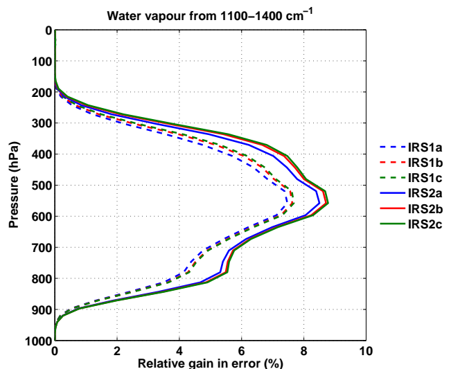
Figure 7. Impact of spectral resolution and radiometric noise on the retrieval of water vapour profile based on the use of the 1100–1400 \text{cm}^{-1} spectral band. The relative gain in error is defined as the difference between the a priori and a posteriori error, divided by the a priori error, averaged over the whole tropical TIGR situations.
