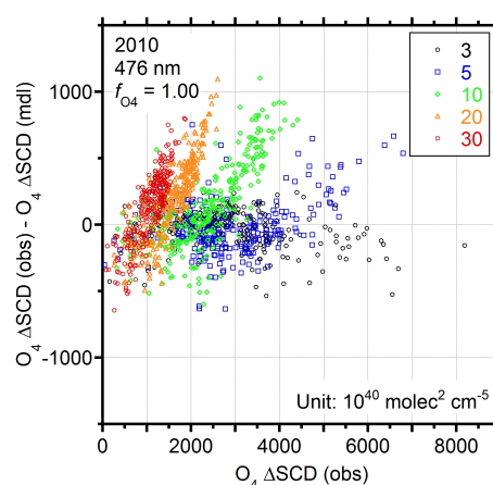
Figure 9. Individual profile retrieval residuals, O_4 \Delta\text{SCD}(\text{obs}) minus O_4 \Delta\text{SCD}(\text{mdl}) , as a function of O_4 \Delta\text{SCD}(\text{obs}) . Values for retrievals with f_{O_4} = 1.00 are plotted. Values for \alpha of 3^\circ , 5^\circ , 10^\circ , 20^\circ , and 30^\circ are shown in black, blue, green, orange, and red, respectively.
