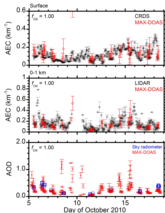
Figure 6. Same as Fig. 4, but a f_{\text{O}_4} of 1.00 is assumed in the MAX-DOAS retrieval.
