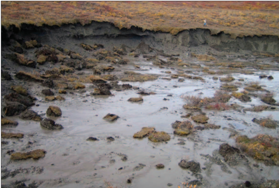
Wulik river slump. David Harbke.
