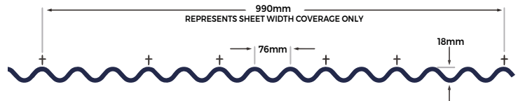
Permissible downward (imposed) loads in kN/m 2
