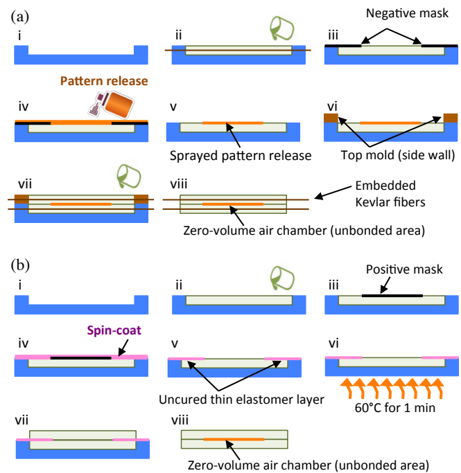
Fig. 3. (a) Fabrication process for a flat pneumatic artificial muscle actuator with a zero-volume air chamber using a negative mask and pattern release (i: Prepare a bottom mold, ii: Pour liquid elastomer for a bottom layer and embed Kevlar fibers, iii: Place a negative mask, iv: Spray pattern release, v: Remove the mask, vi: Place a top mold, vii: Pour liquid elastomer for a top layer and embed Kevlar fibers, and viii: Remove the top and bottom molds when the elastomer cures.). (b) Alternative fabrication process to make a zero-volume air chamber using a positive mask and spin-coating (i: Prepare a bottom mold, ii: Pour liquid elastomer for a bottom layer, iii: Place a positive mask, iv: Spin coat liquid elastomer, v: Remove the mask, vi: Partial bake, vii: Laminate a cured top layer, and viii: Remove the top and bottom molds when the elastomer layers bond with cure.).
