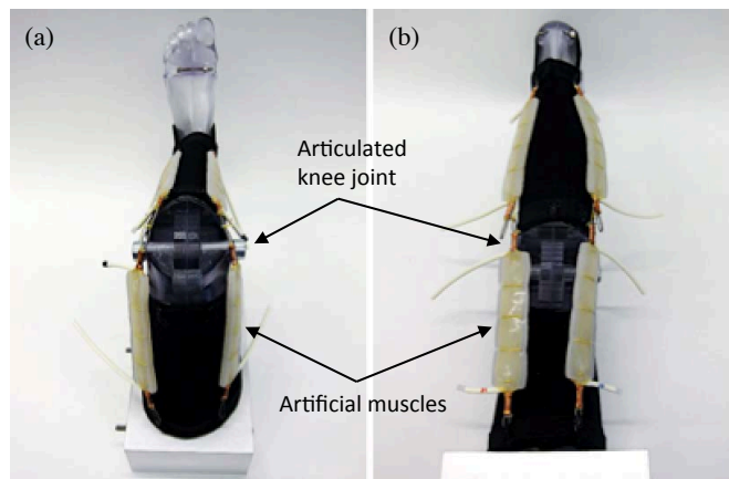
Fig. 6. A complete Second Skin prototype with artificial muscle installation. (a) Anterior side. (b) Posterior side.
