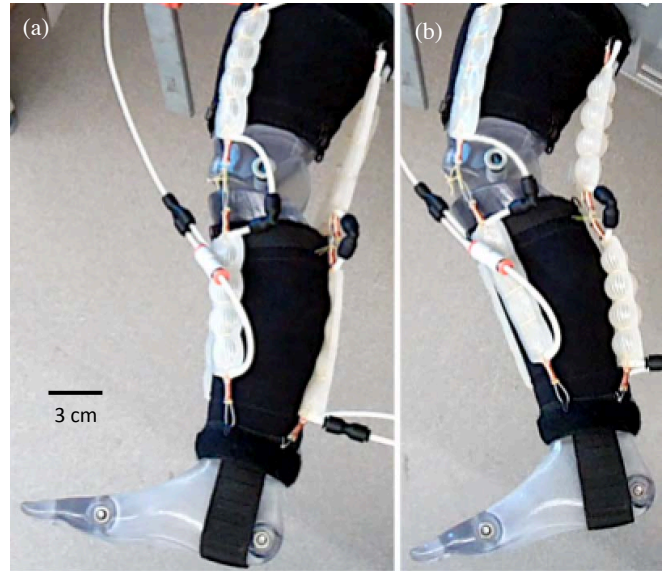
Fig. 1. A Second Skin prototype in action. (a) Active knee extension. (b) Active knee flexion.
