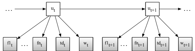
Figure 3: Two consecutive time slices of our dynamic Bayesian network for modeling motion patterns of Twitter users from n friends. All nodes are discrete, shaded nodes represent observed random variables, unshaded denote hidden variables.
