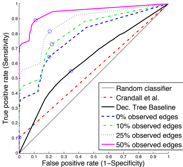
Figure 4: Averaged ROC curves for decision tree baseline, Crandall et al. 's model with the most favorable setting of parameters ( s = 0.001 and t = 4 hours), and Flap.
