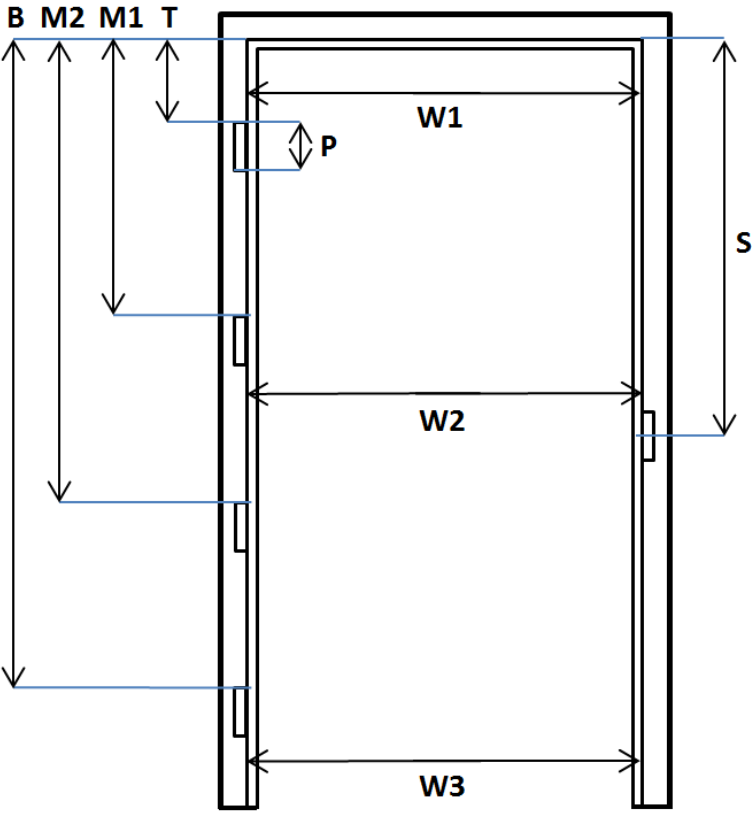
ON FRAME
