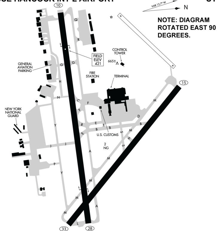
TAXI DIAGRAM
