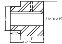
Square Bore with Set Screws
