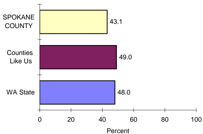
Percent of Traffic Fatalities that are Alcohol-related
