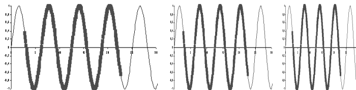
Fig. 2: curvilinear distance on a spiral for different scaling
