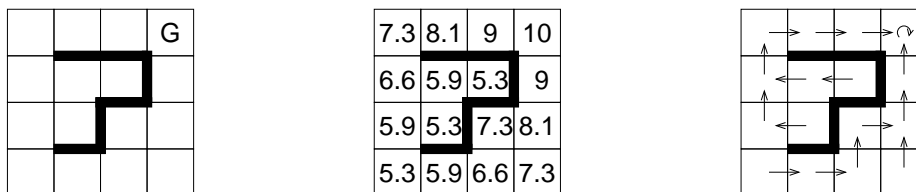
Fig. 1: Example of a simple maze world (left): a robot can move in a world of 16 states choosing actions for going up, down, left, right or stay in the current state. If it stays in the goal state (G) it will obtain a reward of 1, if it collides with a wall or tries to leave the grid world, it will get reward -1 , and in all other cases reward 0. The robot starts in an arbitrary state. The figure in the middle shows the optimal value function V^* for this MDP with discount factor \gamma = 0.9 . The figure on the right shows an optimal policy.
