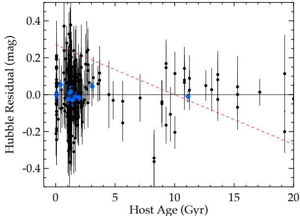
Figure 3. The relationship between the cosmological Pantheon sample’s Hubble-Lemaître residuals and host galaxy age (light-weighted) for the low redshift SNe Ia (black) of Jones et al. (2018). Blue points are bins of 25 SN Ia. Light-weighted ages are biased by bright young stars, reducing the range of observed ages and increasing the measured slope. The red dashed line is the trend seen in K20. The mass step that is applied to the Pantheon Hubble-Lemaître residuals would not drastically shift the trend from K20 because it was derived using only massive early-type galaxies. However, one can easily imagine concluding a low-significance trend if one only used hosts with ages > 2.5 Gyr (the last two bins), as expected in a passive only sample. There appears to be no systemic nor statistical bias in ages values where the K20 regression line would go through this external cosmological data set.
