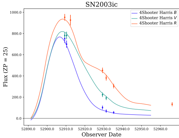
Figure 1. The light curve of SN2003ic. With no pre-maximum data points, it would commonly be removed from cosmological samples due to difficulties constraining the peak luminosity. However this SN Ia alone takes the correlation seen in K20 from a 1.8\sigma to a 2.3\sigma significance. Original photometry from Hicken et al. (2009) .
