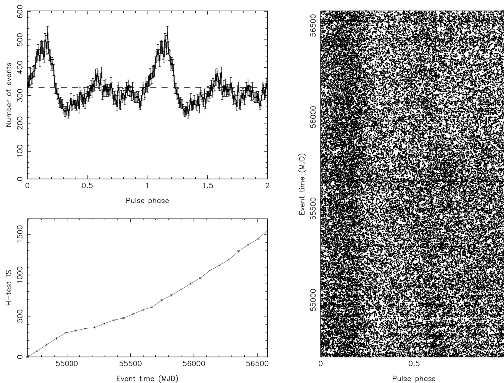
Figure C.5: Tempo2 phase outputs for PSR J2021.5+4026. The top left shows the number of events per phase, the bottom left shows the significance growing with observation time, and the right shows the phased events.
