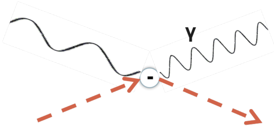
Figure 2.5: Diagram of Inverse Compton scattering, in which a low energy photon interacts with a high-energy electron and is scattered to gamma-ray energies.
