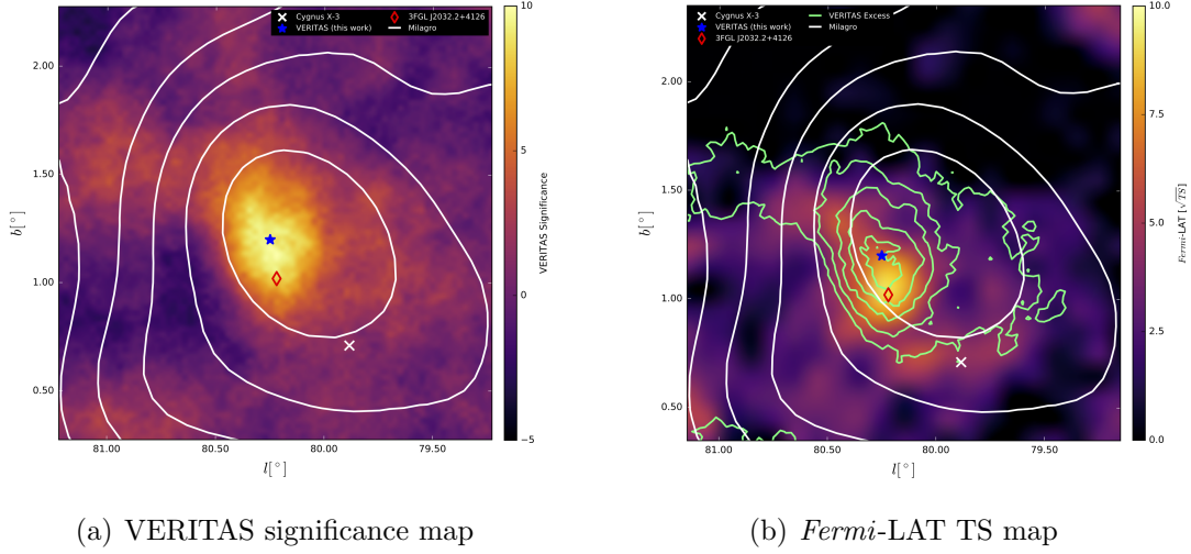
Figure 7.19: (a) The significance map of VER J2031+415. The Milagro: 3, 4, 5, 6, and 7 \sigma contours are plotted in white, along with the locations of other objects of interest. (b) The Fermi -LAT TS map of the residual source that results from the pulsed analysis, with the same Milagro contours, in white, and sources of interest, as well as the 50, 100, 150, 200, and 250 excess contours for the VERITAS source in green.
