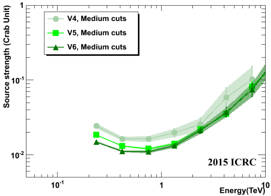
Figure 5.10: A plot of the the VERITAS array sensitivity for different phases of the experiment. V4 refers to the original array configuration, V5 to the array post-T1 move, and V6 to the array with the camera upgrade. The source strength is calculated as a percentage of the flux of the Crab Nebula in a given energy bin such that the source would be detected with 5\sigma significance after 50 hours of observing time. Figure from [97].
