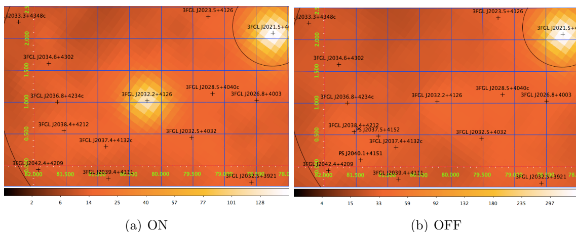
Figure C.6: Zoomed in counts map of PSR J2032.2+4126 region (square root scale, smoothed by 3 pixels). On the left is the counts in the on phase and on the right is the counts in the off phase.
