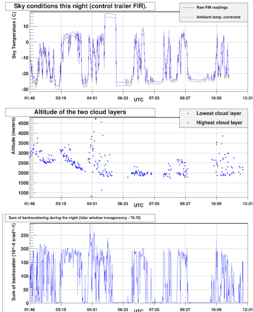
Figure 5.7: Weather data from a cloudy night at VERITAS. The top panel shows the output from the infrared sky temperature monitor, the middle panel shows the output from the LIDAR measurement of the height of the clouds, and the bottom panel shows the LIDAR measurement of the transparency of the clouds.
