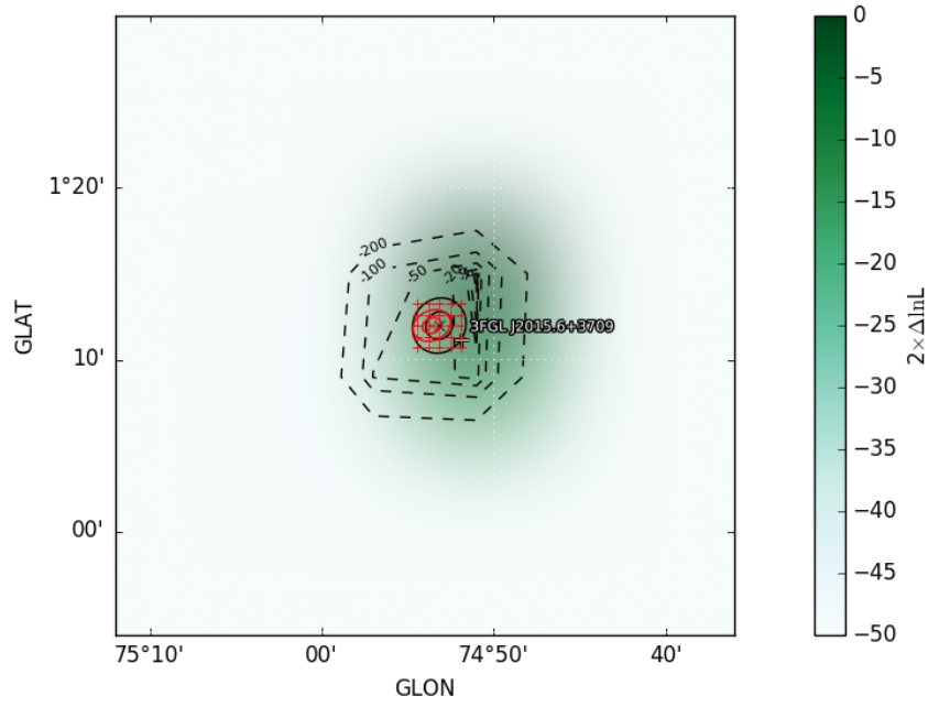
Figure 7.26: The Fermi -LAT TS map of 3FGL J2015.6+3709 (CTB 87). The counts contours are labeled. Marked is the 3FGL J2015.6+3709 source position and the best fit position, which is slightly offset toward CTB 87.
