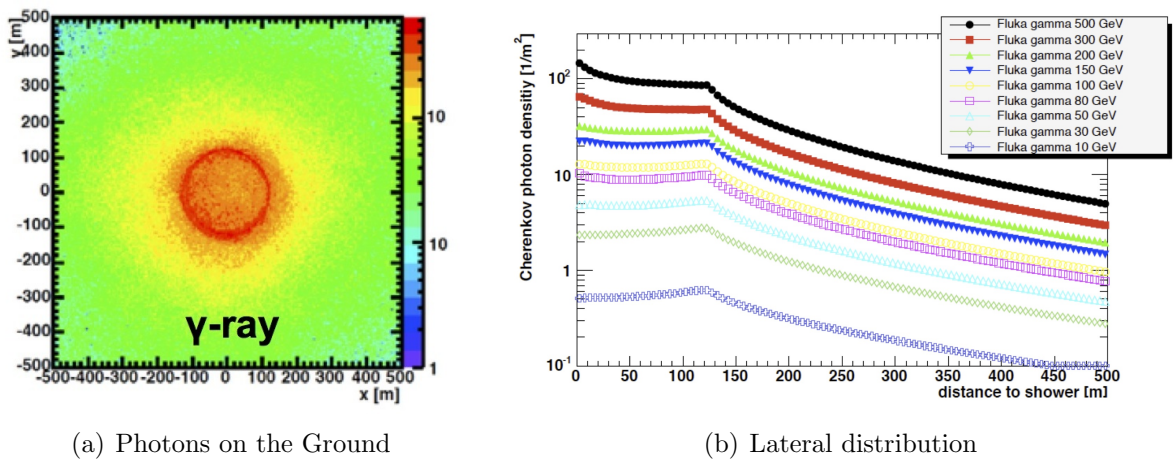
Figure 4.7: (a) Simulated Cherenkov photon density at VERITAS ground level (1.3 km a.s.l.) for a 1 TeV primary. The Cherenkov photon density, in units of photons per m^2 , are plotted in the color scale as a function of x-y position on the ground in meters. (b) Average lateral distribution for showers produced by primary gamma rays of different energies. Figure from the VERITAS collaboration.
