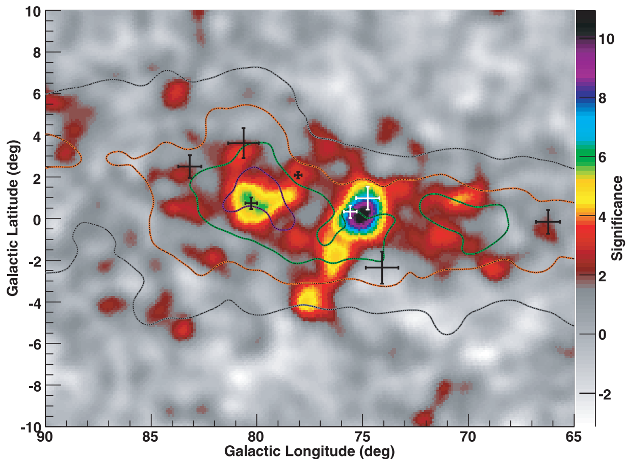
Figure 3.3: The Milagro map of the Cygnus region of the Galaxy. The color bar is in units of significance in standard deviations. The contours trace matter in the region from CO and HII surveys of the region. The crosses indicate EGRET sources. The large region with high significance is associated with MGRO J2019+37, and the smaller region to the left, with lower significance, is associated with TeV J2032+4126. Figure from [77].
