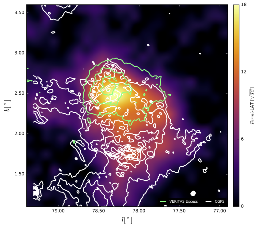
Figure 7.21: Fermi -LAT TS map (in color) of the region around VER J2019+407 with the pulsar source and nearby sources included in the model. The VERITAS excess contours are overlaid in green and the CGPS radio contours in white [132]. The Fermi -LAT and radio contours are well matched and are peaked with the VERITAS source.
