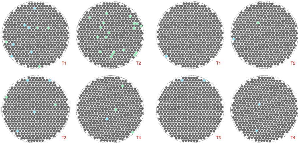
Figure 5.9: The dead channels pre- (left), and post- (right) PMT upgrade for each camera (TX, where X ranges from one to four is the label given to each telescope). The good channels are in gray, with dead channels in light blue [100].
