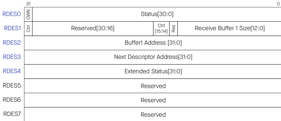
Figure 10-10. Receive Descriptor
