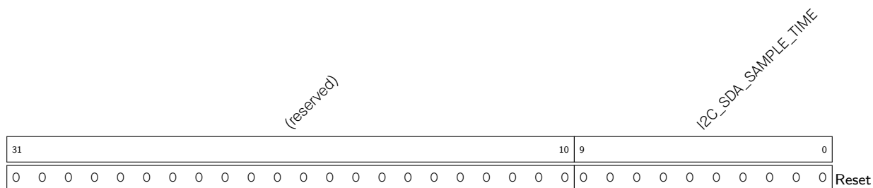
Register 11.13. I2C_SDA_SAMPLE_REG (0x0034)
