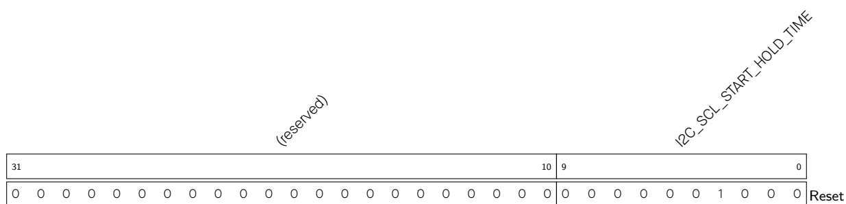
Register 11.15. I2C_SCL_START_HOLD_REG (0x0040)
