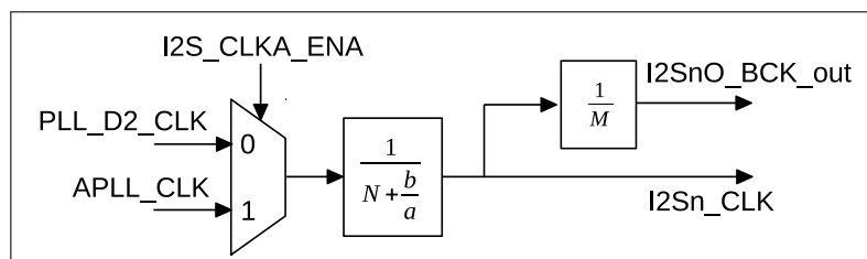
Figure 12-2. I2S Clock
