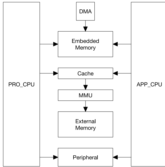
Figure 1-1. System Structure
