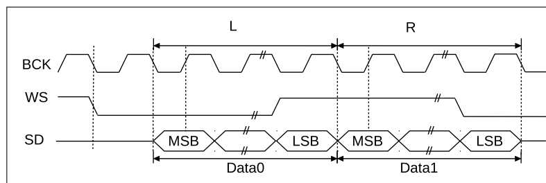
Figure 12-3. Philips Standard
