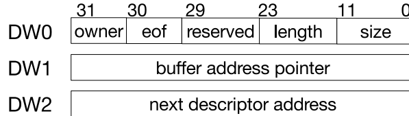
Figure 6-2. Linked List Structure
