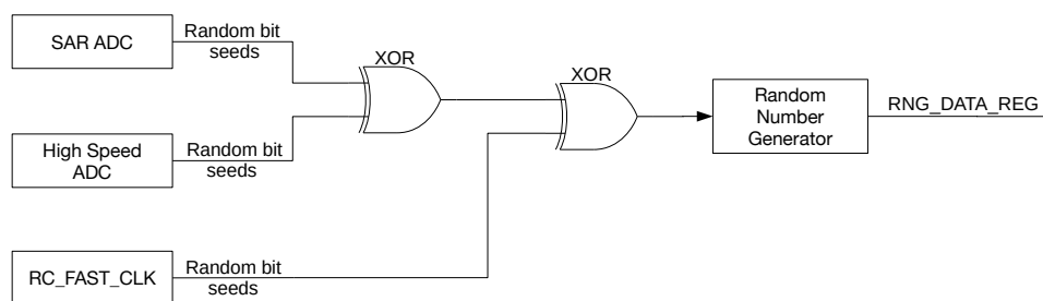
Figure 25-1. Noise Source
