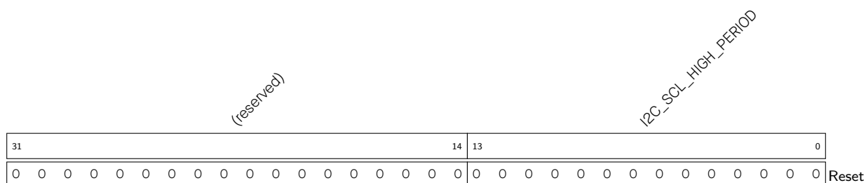
Register 11.14. I2C_SCL_HIGH_PERIOD_REG (0x0038)
