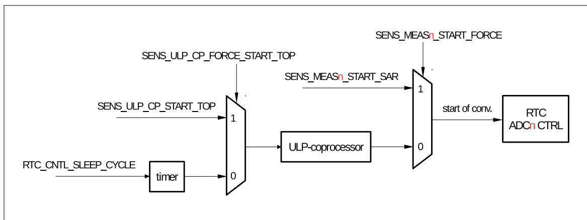
Figure 29-7. RTC SAR ADC Outline of Function
