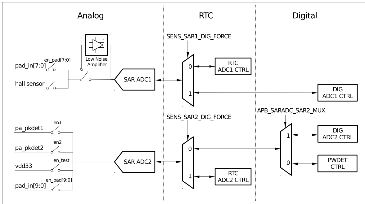
Figure 29-6. SAR ADC Outline of Function
