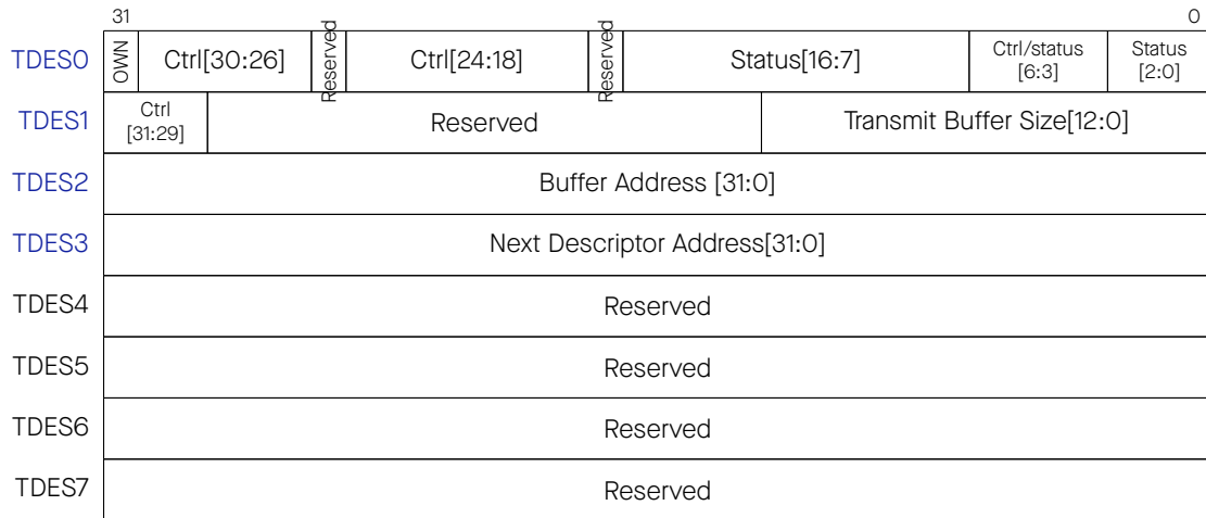
Figure 10-9. Transmit Descriptor
