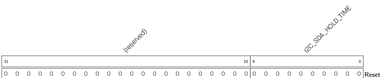
Register 11.12. I2C_SDA_HOLD_REG (0x0030)
