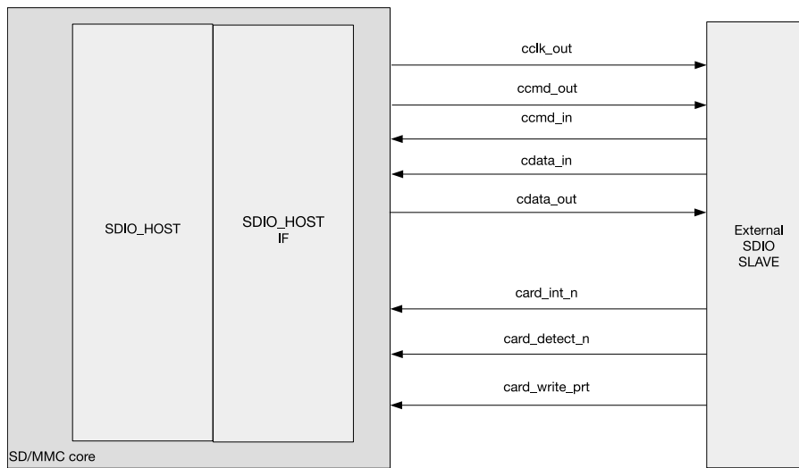
Figure 9-2. SD/MMC Controller External Interface Signals
