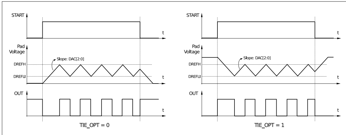
Figure 29-3. Touch Sensor Operating Flow
