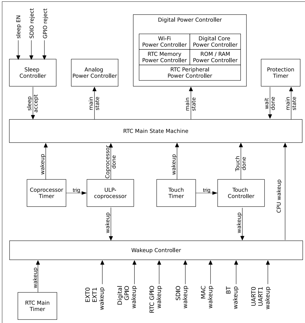
Figure 31-6. RTC Structure
