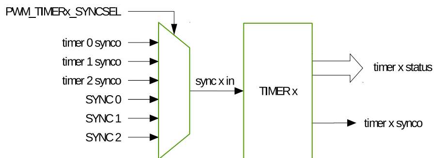
Figure 16-3. Timer Submodule
