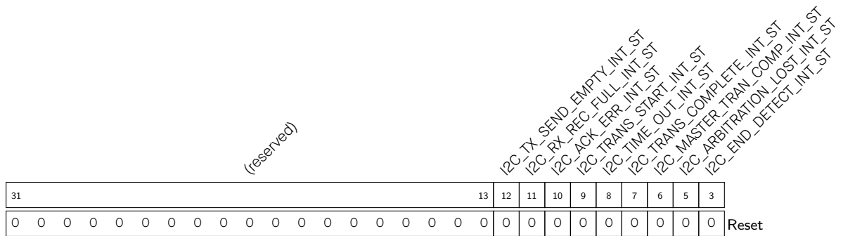
Register 11.11. I2C_INT_STATUS_REG (0x002c)
