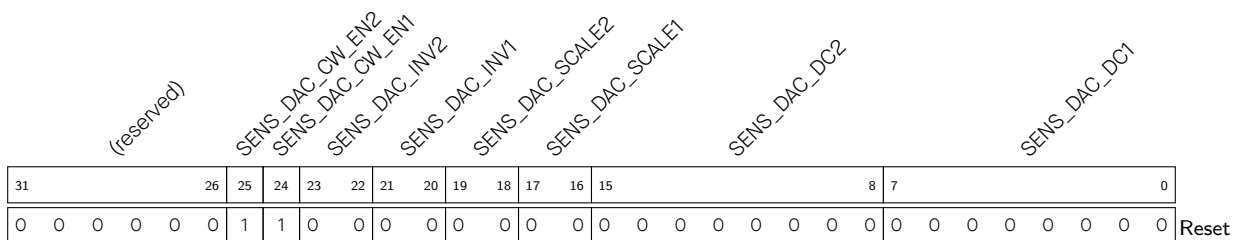
Register 29.23. SENS_SAR_DAC_CTRL2_REG (0x009c)
