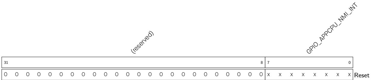
Register 4.27. GPIO_ACPU_NMI_INT1_REG (0x0078)
