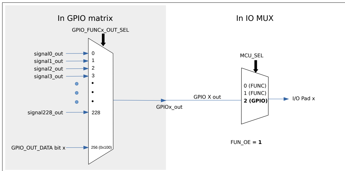
Figure 4-4. Output via GPIO Matrix
