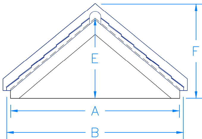
Front Elevation
