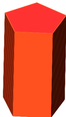
Pentagonal Prism
