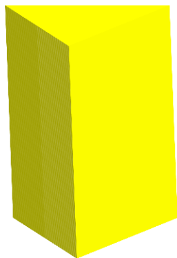
Triangular Prism
