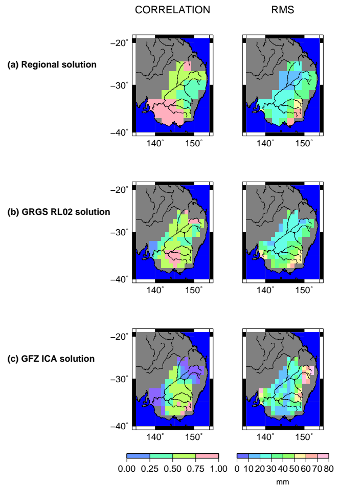
Fig. 16. Spatial correlation (left maps) and RMS (right maps) of differences between TWS (in situ GWS measurements + surface water + modelled soil moisture) and: (a) regional solutions, (b) GRGS RL02 solutions and (c) ICA 400 km-filtered solutions.
