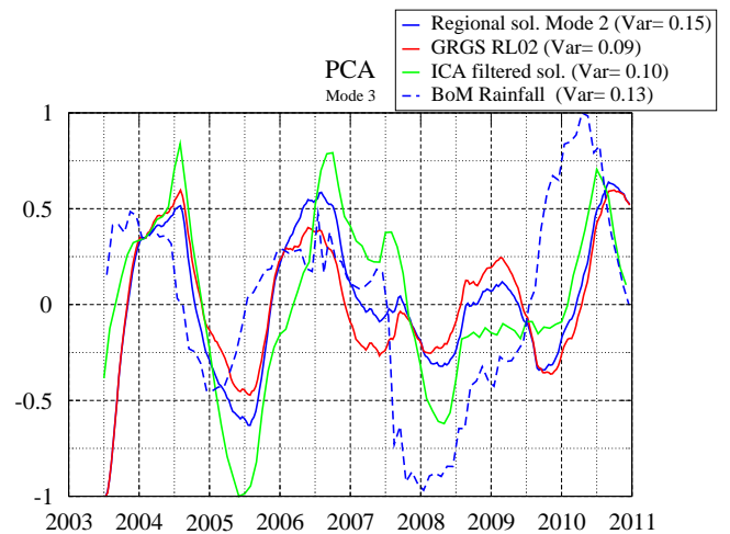
Fig. 11. Temporal components of PCA 2nd orthogonal mode of regional solutions and 3rd mode of GRGS, ICA 400 km-filtered solutions and rainfall product.
