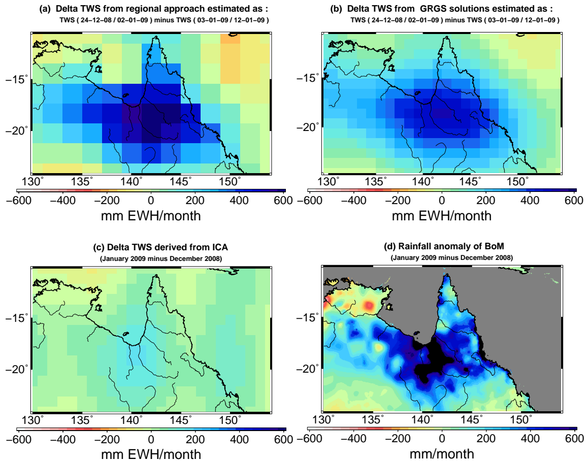
Fig. 13. \Delta TWS time series map derived from regional solutions (a), from GRGS RL02 (b), from ICA-filtered solutions (c) and rainfall anomalies for January 2009 (d). We notice in January solutions the strong amplitudes in the Gulf of Carpentaria due to the floods caused by cyclone Charlotte (9 January–12 January 2009).
