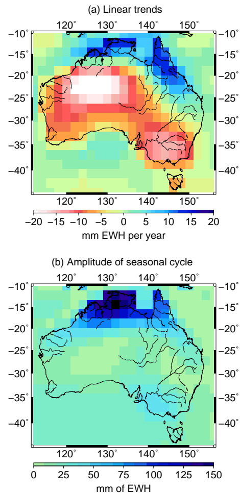
Fig. 4. (a) Linear trends and (b) annual amplitudes derived from GRACE-based regional solutions for 2003–2009.
