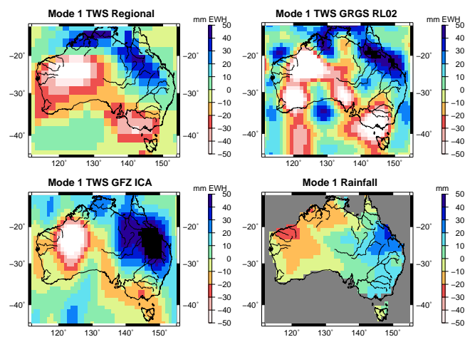
Fig. 6. Spatial components of PCA 1st orthogonal mode.
