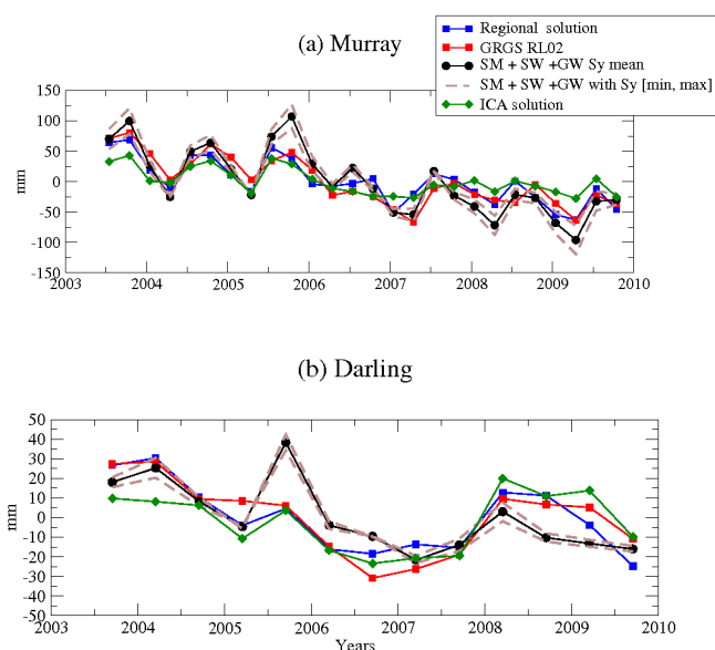
Fig. 15. (a) 3-month averaged time series of TWS over Murray Basin and (b) 6-month averaged time series of TWS over Darling Basin for 2003–2010. Series are computed from GRACE-based regional solutions (blue line), GRGS RL02 (red line), ICA 400 km-filtered solutions (green line) and TWS estimated as groundwater storage + surface water observations + modelled soil moisture (grey/black lines). Discontinuous grey line: maximum and minimum values of the specific yield are used; continuous black line: mean value of specific yield is used.
