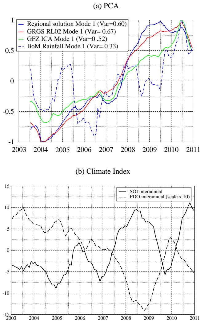
Fig. 7. (a) Temporal components of PCA 1st orthogonal mode. (b) Interannual variations of the Southern Oscillation Index (SOI) and Pacific Decadal Oscillation (PDO).
