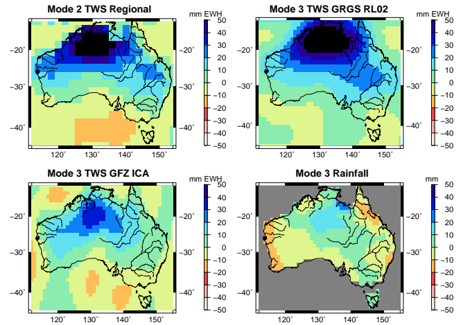
Fig. 10. Spatial components of PCA 2nd orthogonal mode of regional solutions and 3rd mode of GRGS, ICA 400 km-filtered solutions and rainfall product.
