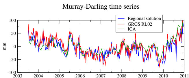
Fig. 14. 10-day and monthly time series of averaged total water storage over the whole Murray–Darling Basin from 2003 to 2011 computed from 10-day regional solutions (blue line), 10-day GRGS global solutions (red line) and monthly ICA 400 km-filtered solutions (green line).
