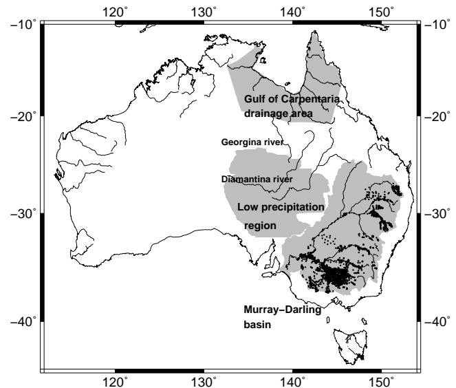
Fig. 1. Australian drainage regions used in our study. Geographical locations of the bores in the Murray–Darling are marked as black circles. They represented, with at least 60 % of data period populated (because of their availability during the period 2002–2009), averages of the first 30 m of the water column height.
