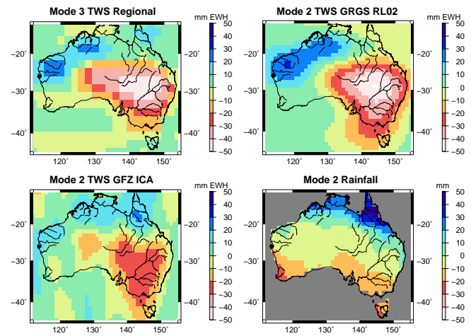
Fig. 8. Spatial components of PCA 3rd orthogonal mode of regional solutions and 2nd mode of GRGS, ICA 400 km-filtered solutions and rainfall product.
