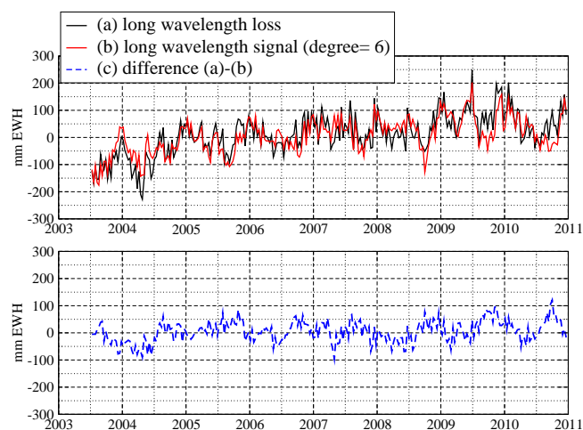
Fig. 2. Water mass time series averaged over Australia: (a) difference between regional and GRGS solutions, (b) GRGS GRACE solutions up to degree 6, and (c) their difference (RMS value 39 mm).
