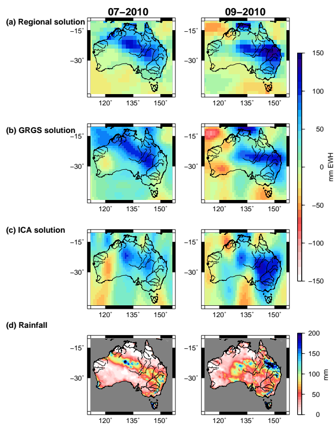
Fig. 12. Regional and GRGS RL02 of \Delta TWS monthly maps estimated with respect to the mean map for the previous driest season (from June to November 2009), and rainfall maps. For these two periods we notice that the regional solutions show a better localization of the exceptional rainfall maximum occurring in the central region of Australia.
