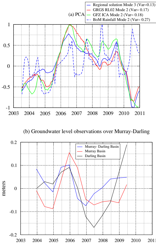
Fig. 9. (a) Temporal components of PCA 3rd orthogonal mode of regional solutions and 2nd mode of GRGS, ICA 400 km-filtered solutions and rainfall product. (b) Groundwater levels from in situ measurements over Murray–Darling Basin.
