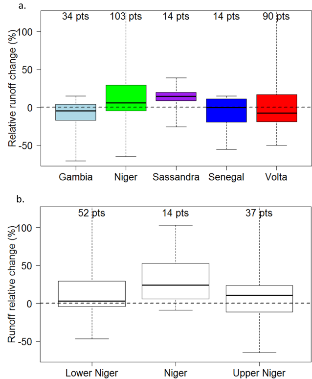
Figure 4. (a) Impact of climate change on runoff (%), by river. Some previous clustering has been done (e.g., Bani and Benue are included with Niger and all the Volta tributaries are together). (b) Runoff relative change (%) for different parts of the Niger River, according to the database. When only Niger is specified, this means that there is no description (upper or lower Niger) in the original paper.
