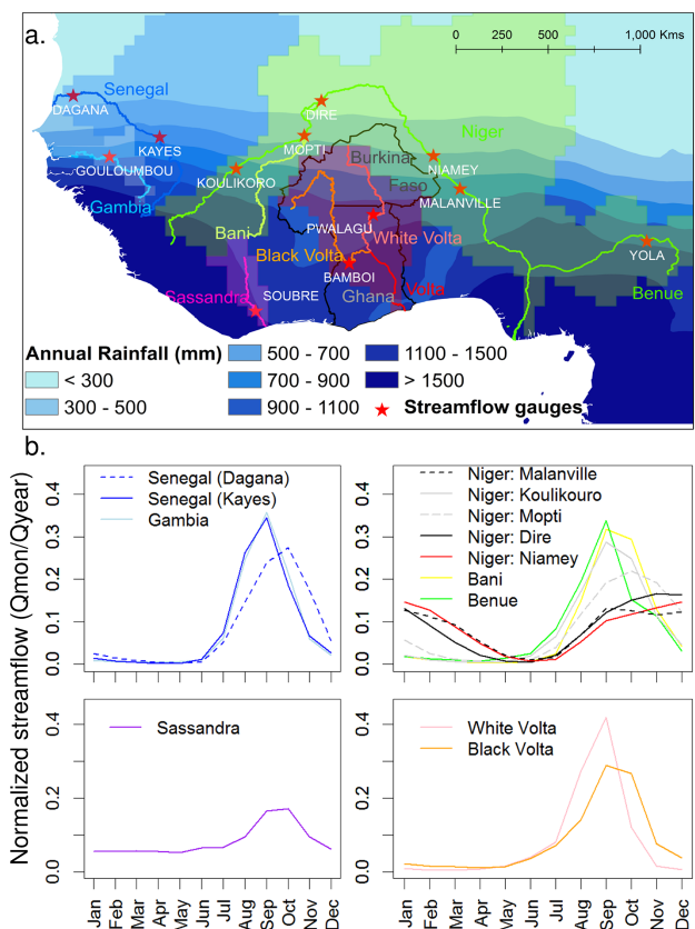
Figure 1. (a) Rivers selected in this study. Rainfall values are from CRU 3.1 data set (1970/2009) (Mitchell and Jones, 2005). Note that White Volta is also named Nakambe River. (b) Mean normalized hydrographs of the studied river basins ( Q_{\text{month}}/Q_{\text{year}} ). Historical data come from the Global Runoff Data Centre (2011) (GRDC) and are for different time periods, depending on the river, but with at least 27 years.
