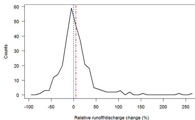
Figure 2. Runoff change ( x axis, %) in WA based on all cases in the database (i.e., including different time period, rivers and models). The blue dashed line represents the median of the distribution; the red one is the mean. We focus here only on the impact of climate change: this is the only changing parameter (no water use or land use change).
