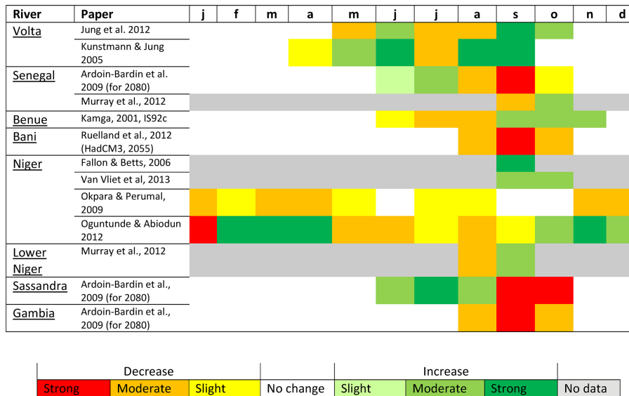
Figure 7. Qualitative assessment of monthly runoff relative change, for different studies of the database and for different rivers. The assessment may be an interpretation of the paper’s results (see Table 4 for more details about each paper results). In some cases we only detailed here one time horizon or one climate model.
