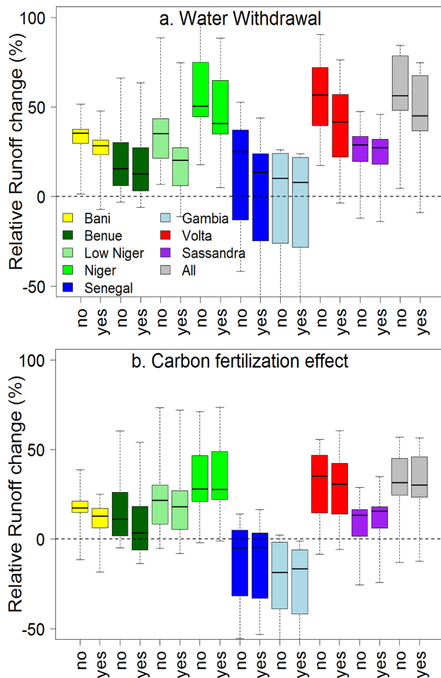
Figure 8. (a) Impact of future water withdrawals on runoff relative change (%) for 8 rivers. (b) Runoff relative change (%) for 8 rivers and 2 different scenarios: (i) taking higher carbon concentration into account (“Yes”) and (ii) with fixed carbon concentration (“No”). Values are from Murray et al. (2012).
