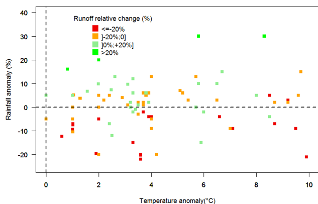
Figure 5. Rainfall (y axis) and temperature (x axis) anomalies associated with the runoff relative change (color scale). All the values come from the database.
