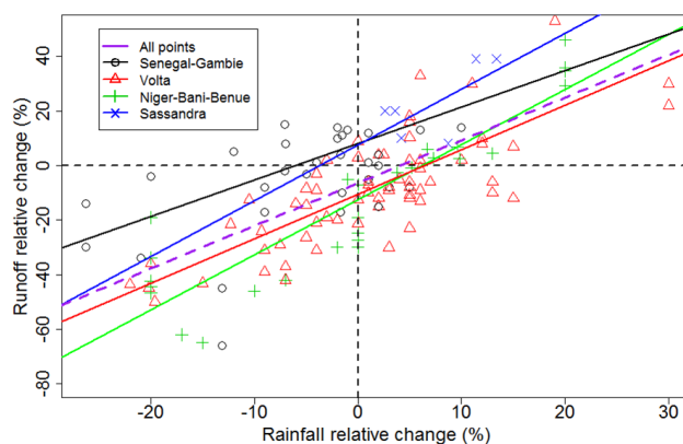
Figure 6. Relationship between runoff change (y axis, %) and rainfall relative change (x axis, %) for the four main rivers and for the whole panel (purple dashes). The lines represent the linear model for each river. Note that we put Senegal and Gambia together.
